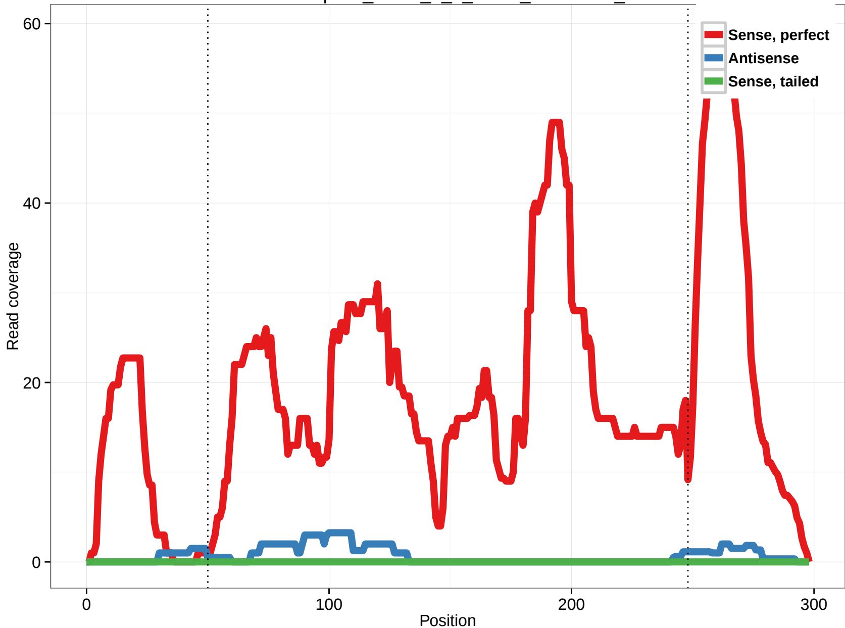
uc002qdz.2_intron_0_0_chr19_54704830_f
