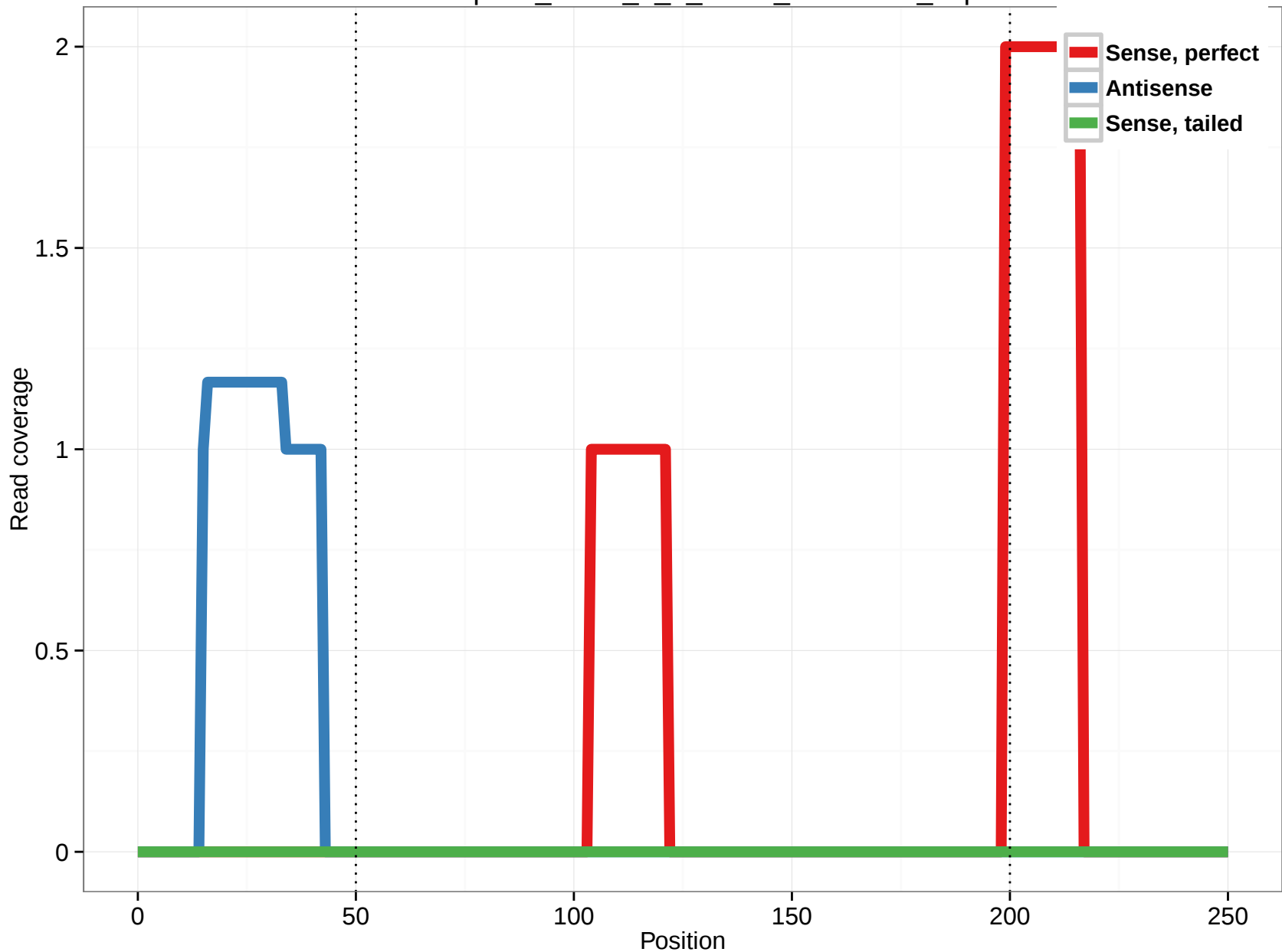
uc002qdh.2_intron_7_0_chr19_54628036_f.3p
