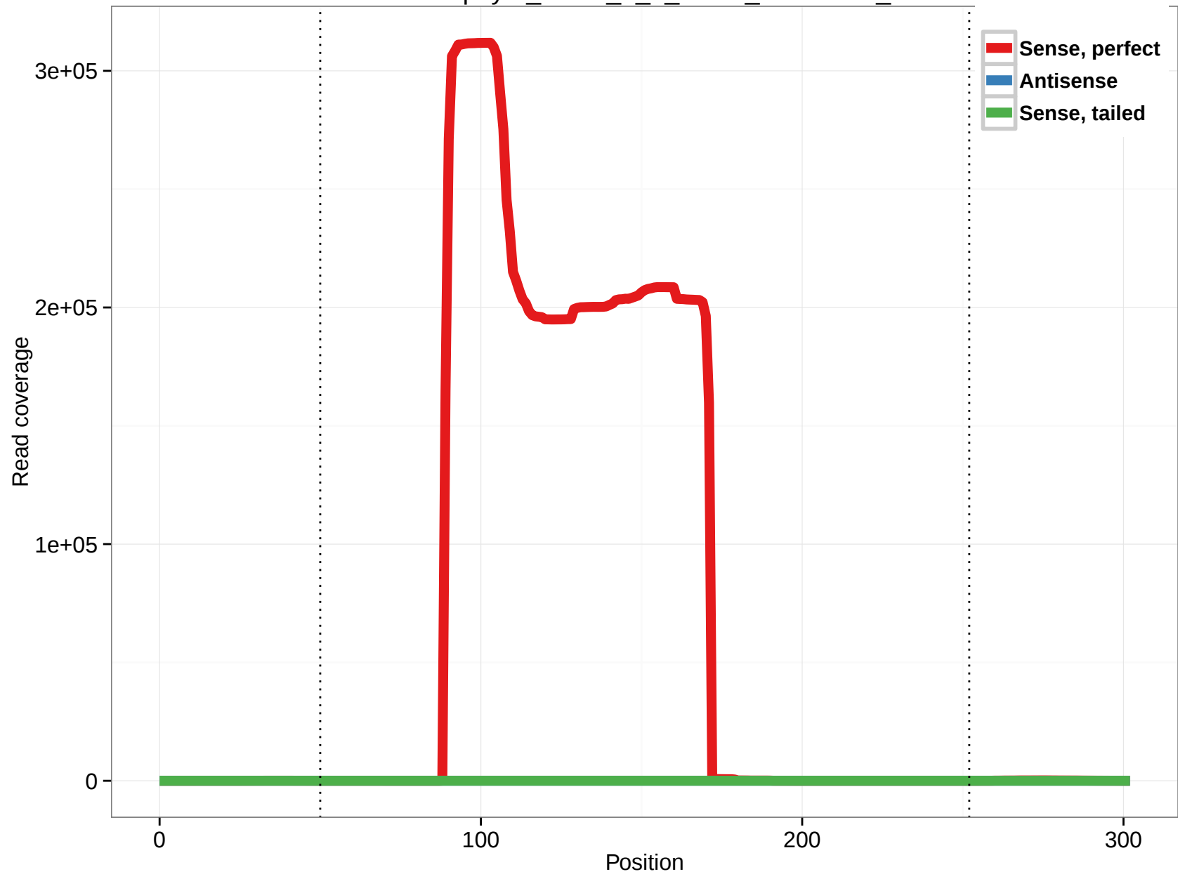
uc002pny.2_intron_3_0_chr19_49993834_f
