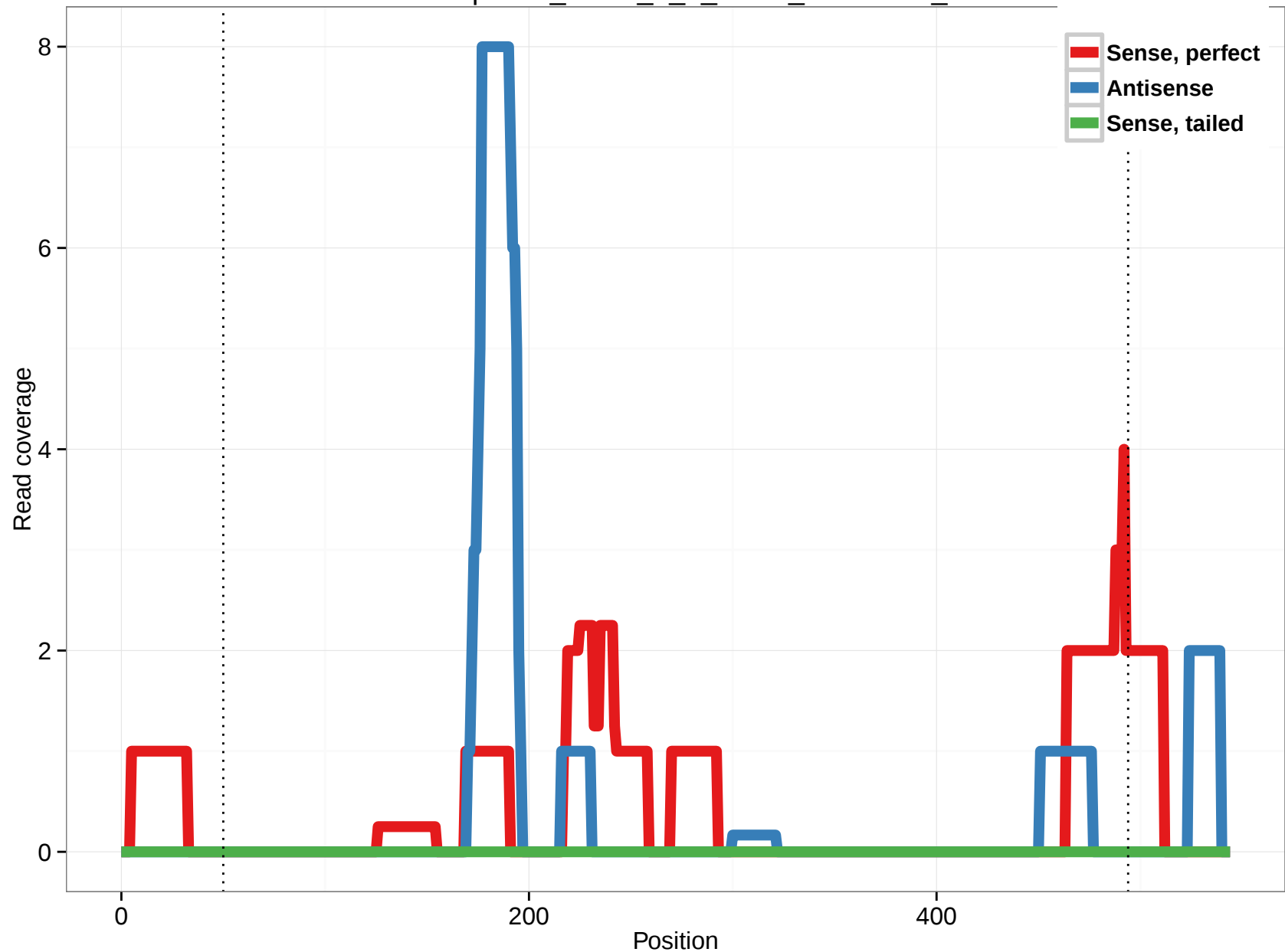
uc002pmz.2_intron_2_0_chr19_49796640_r
