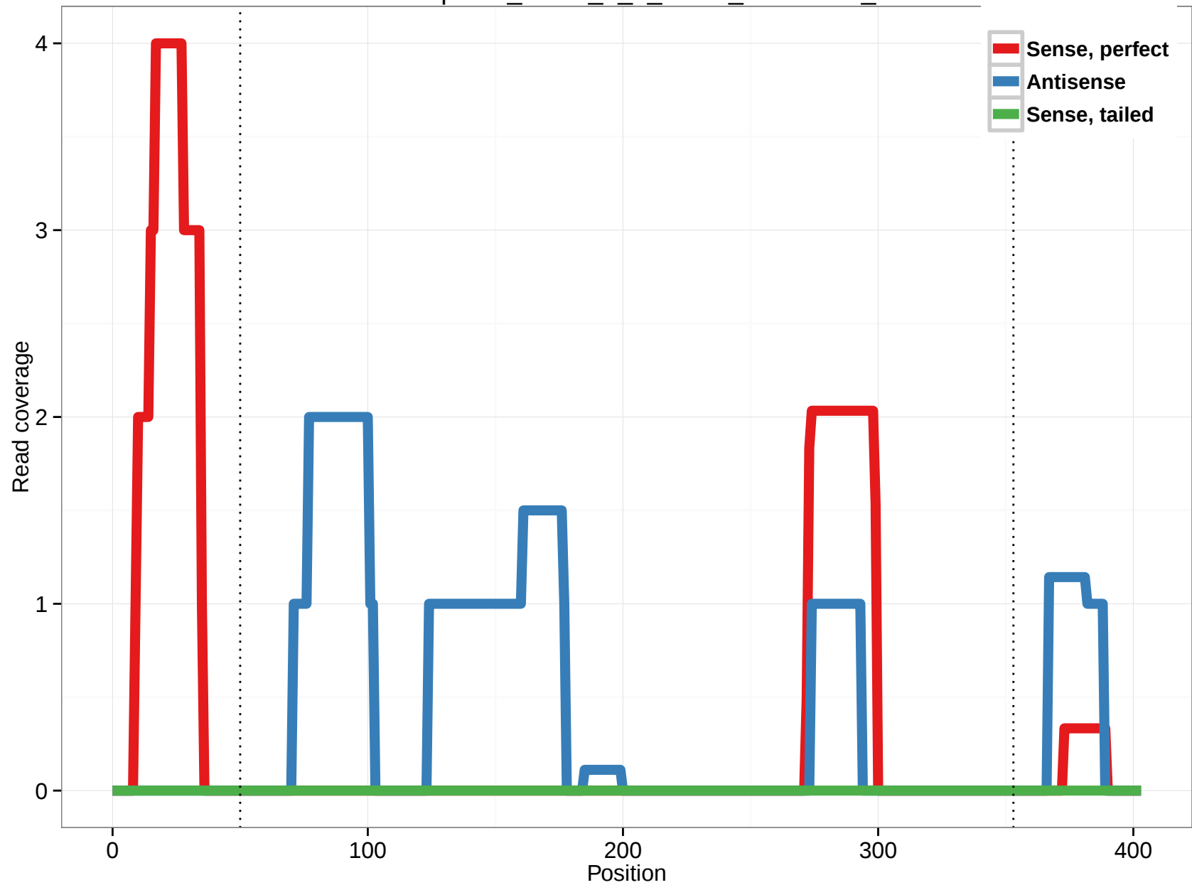
uc002pea.1_intron_2_0_chr19_46627579_r
