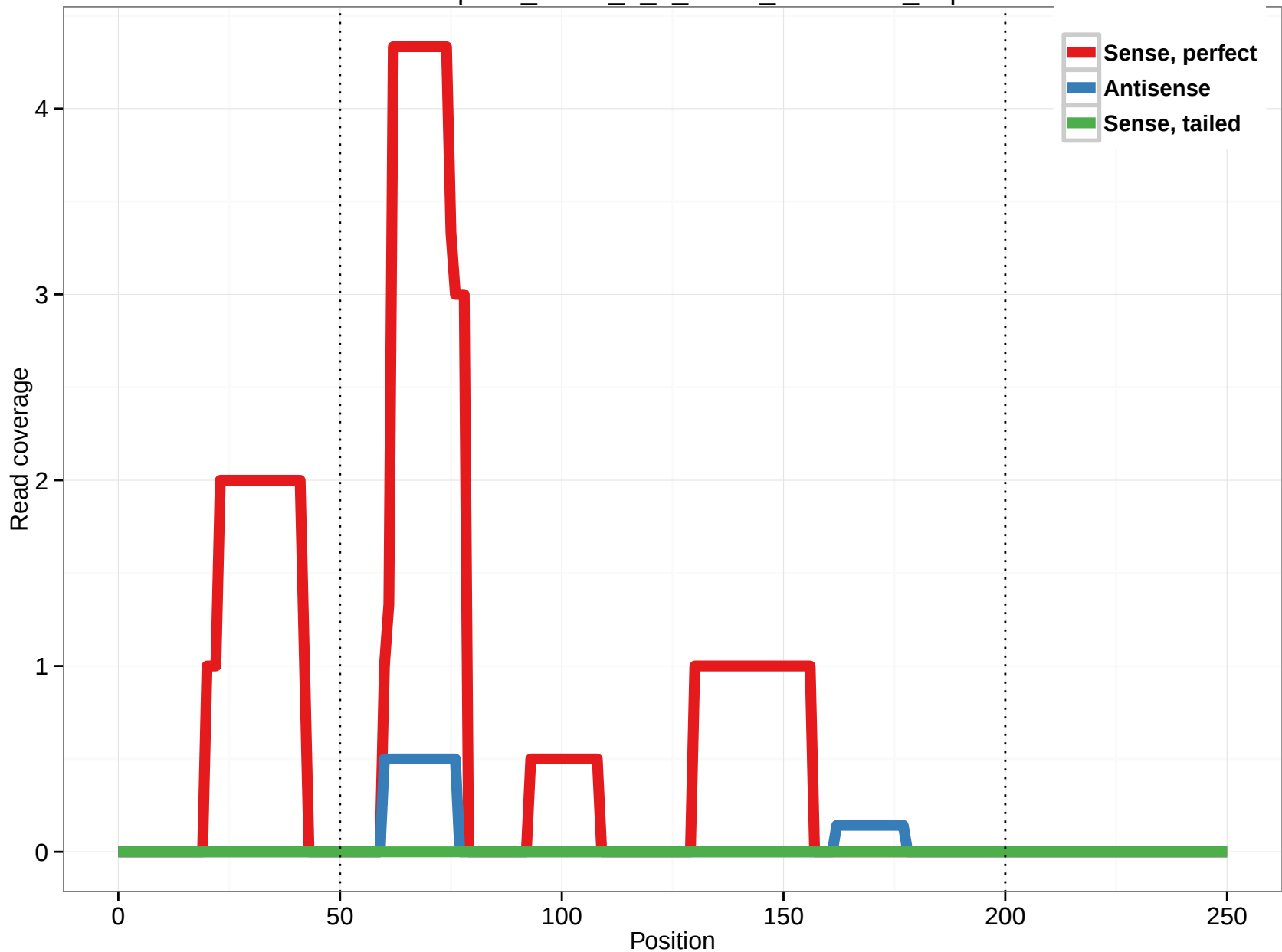
uc002pdr.2_intron_0_0_chr19_46367784_f.5p
