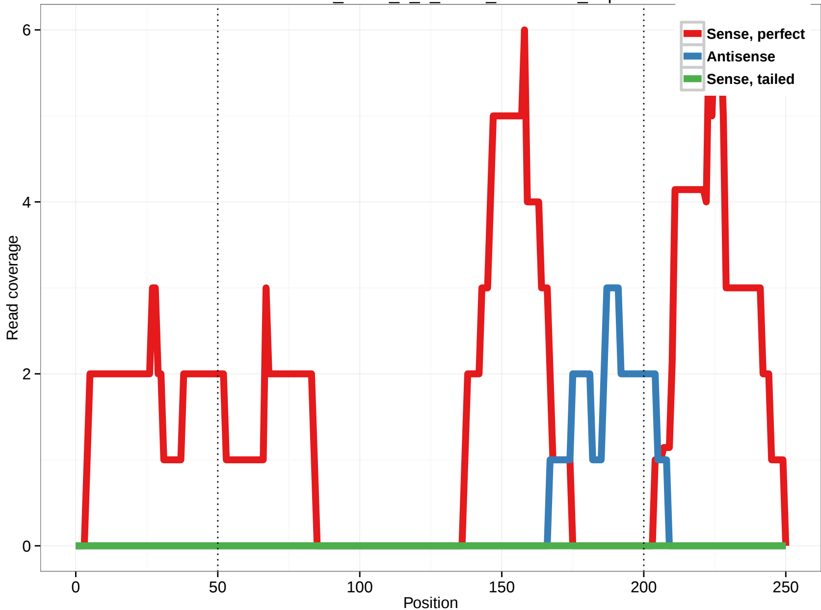
uc002ooi.1_intron_0_0_chr19_41107544_f.3p
