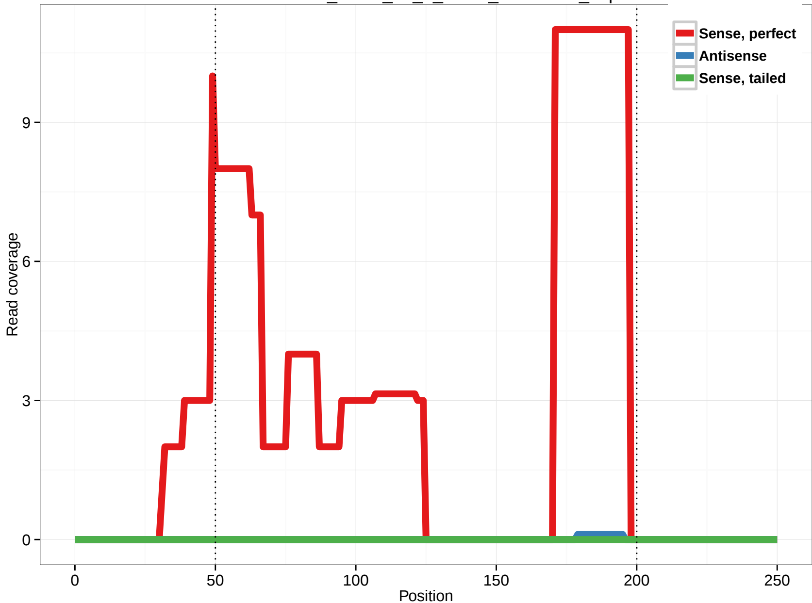
uc002oob.2_intron_14_0_chr19_41095085_f.5p
