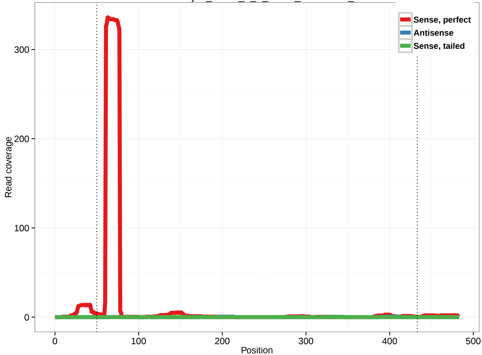
uc002ojf.3_intron_0_0_chr19_39279873_f
