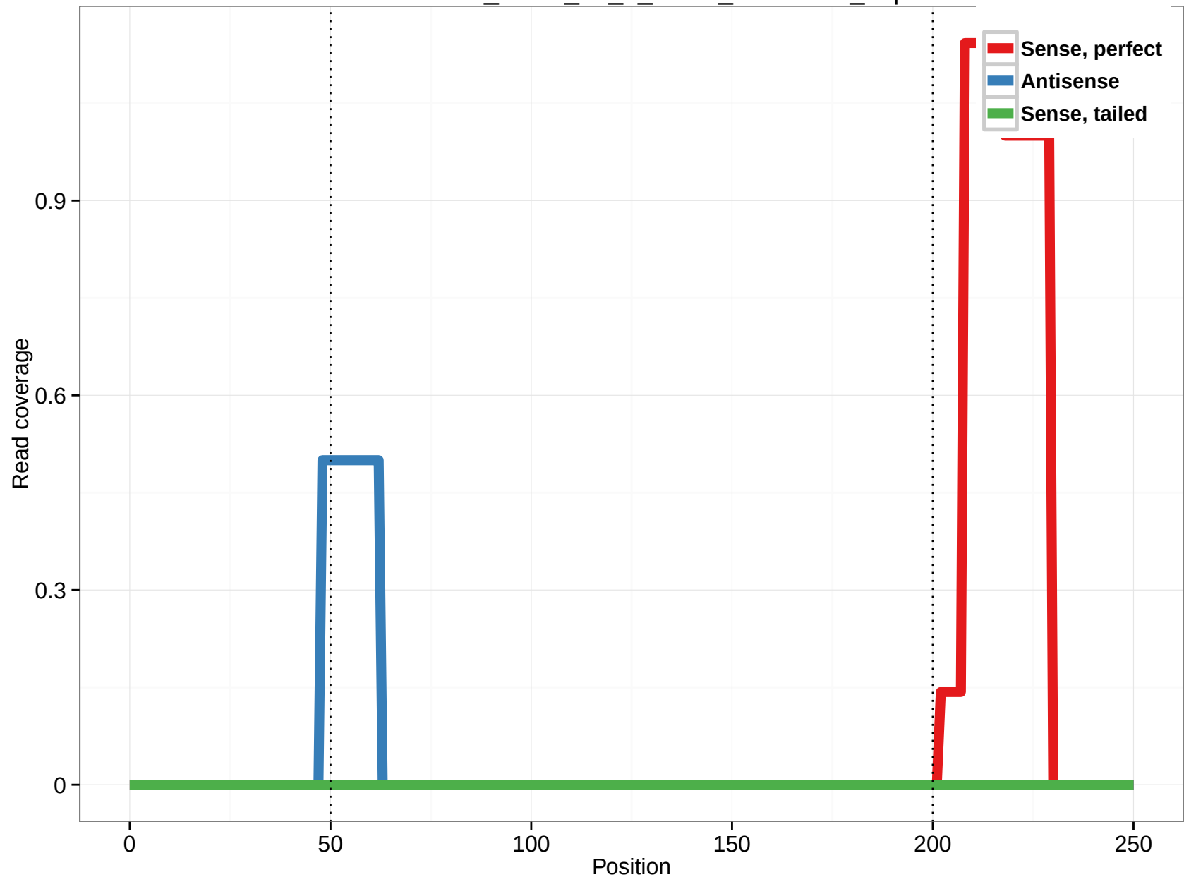
uc002oih.3_intron_21_0_chr19_38855758_f.5p
