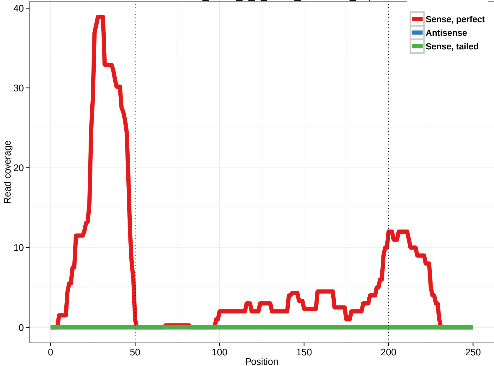
uc002nzi.3_intron_4_0_chr19_35991483_r.5p
