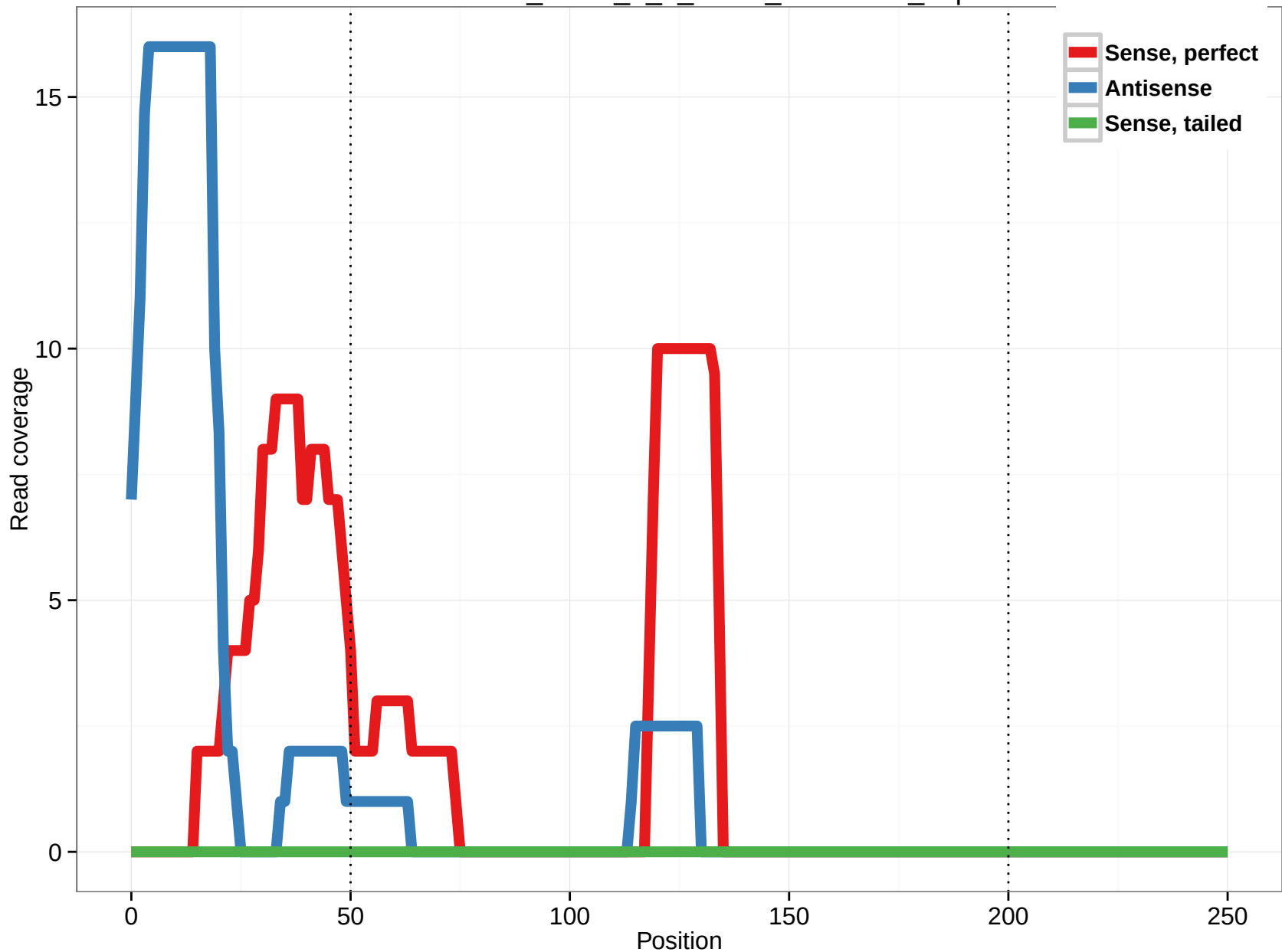
uc002nxf.2_intron_0_0_chr19_35418121_f.5p
