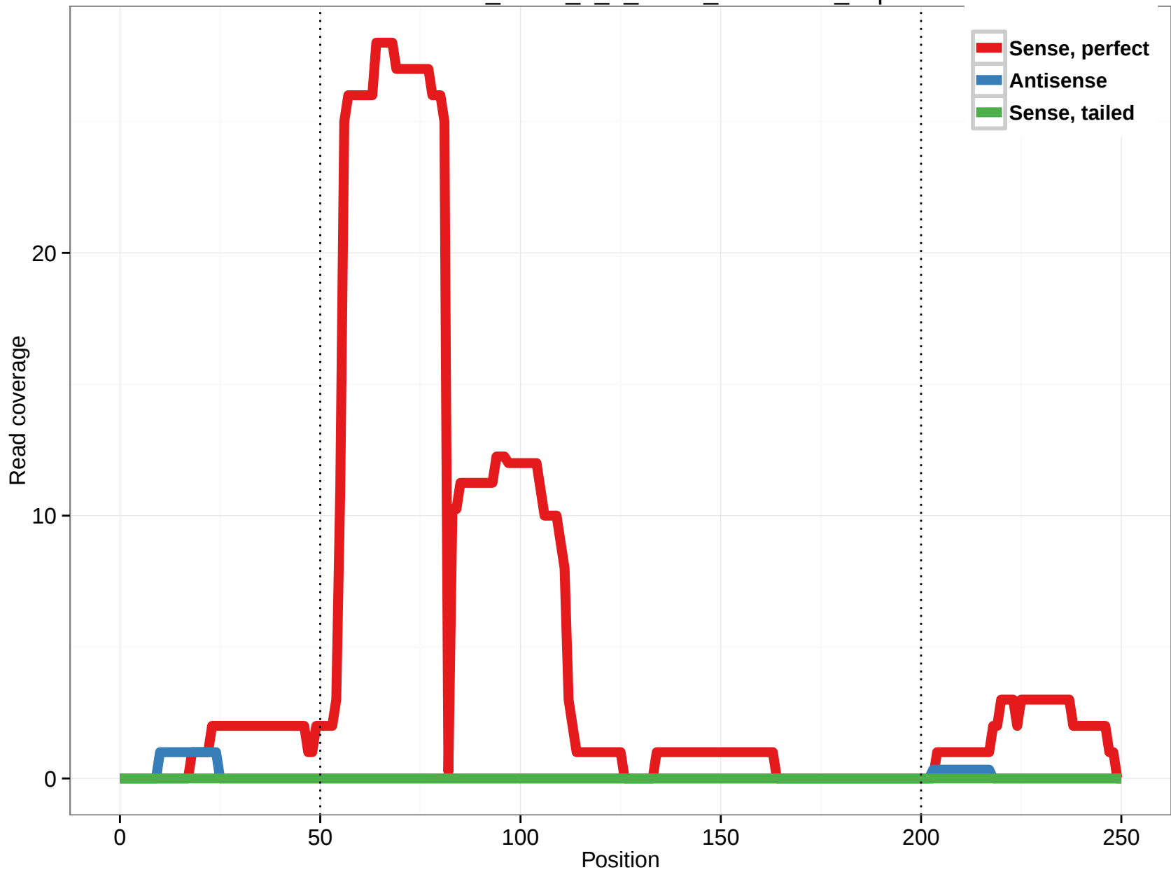
uc002nmt.1_intron_1_0_chr19_19640323_f.3p
