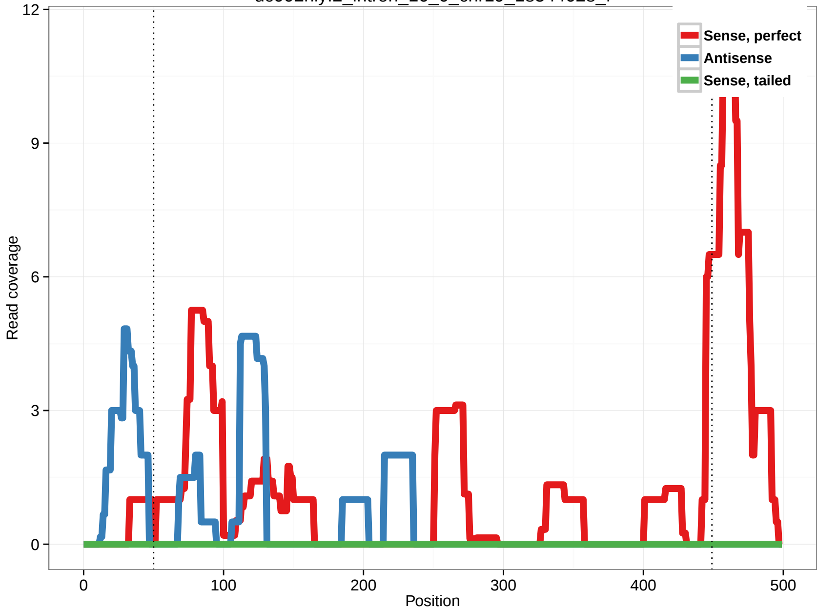
uc002niy.2_intron_16_0_chr19_18544628_f
