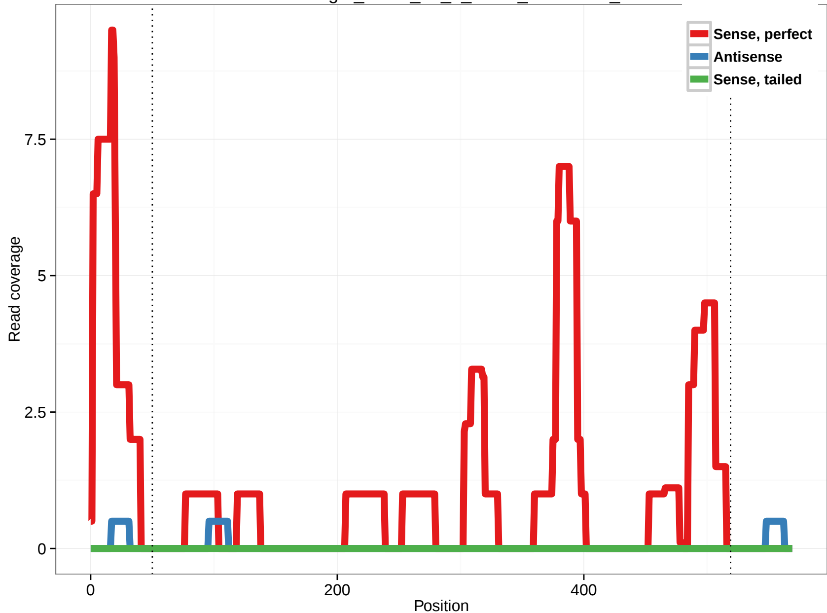
uc002nhg.3_intron_14_0_chr19_17886323_f
