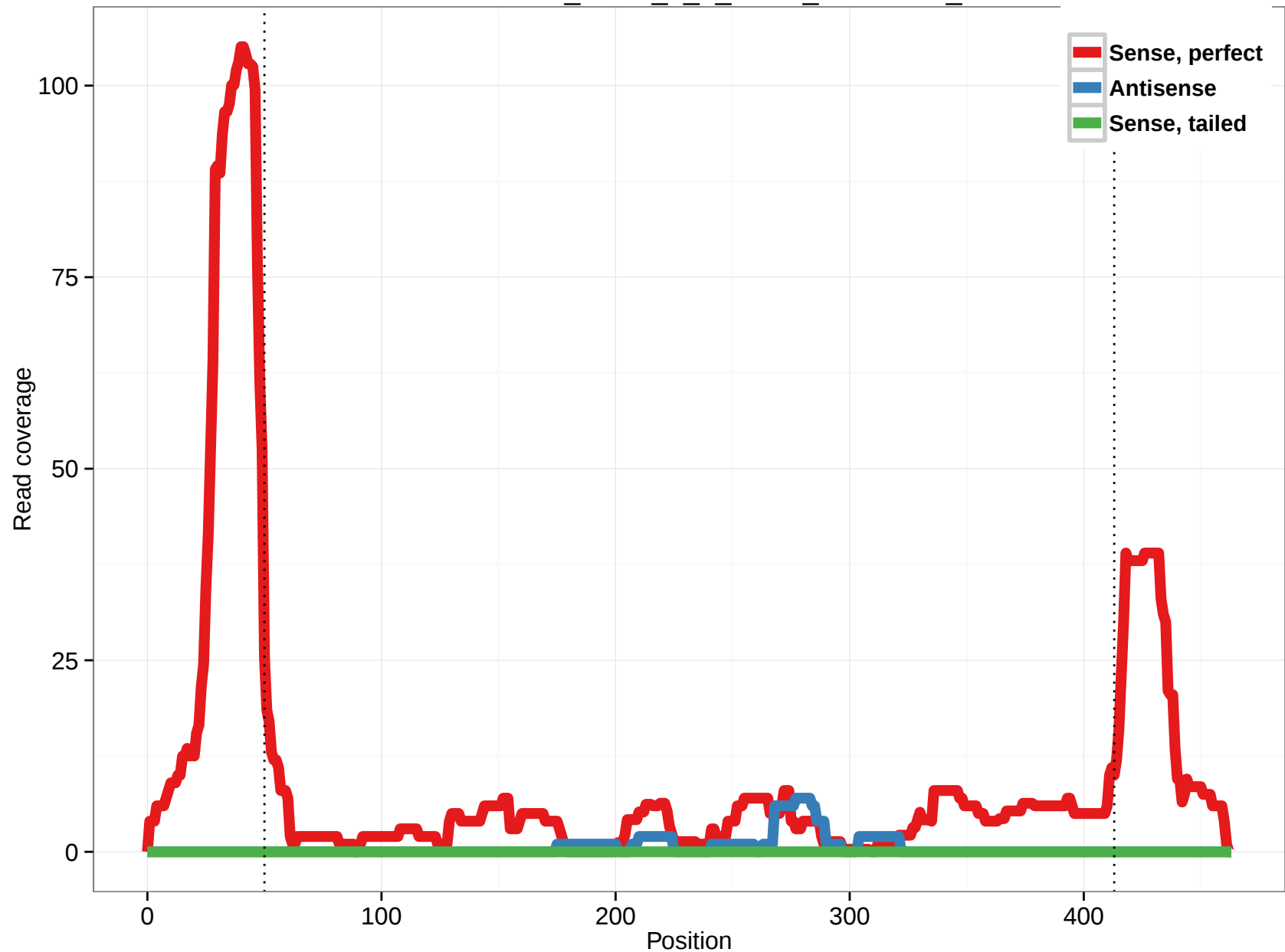
uc002mvu.2_intron_0_0_chr19_13049585_f
