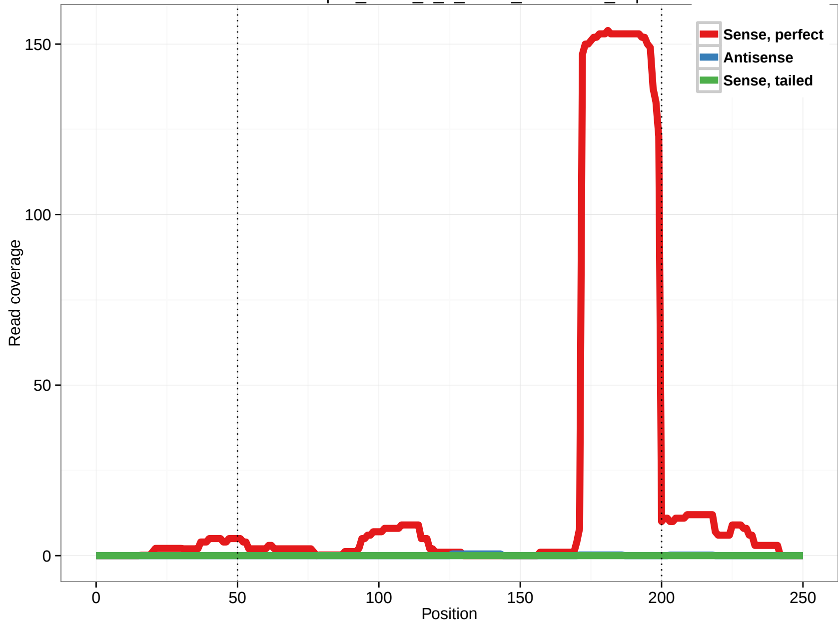
uc002mqe.2_intron_0_0_chr19_11071851_f.3p
