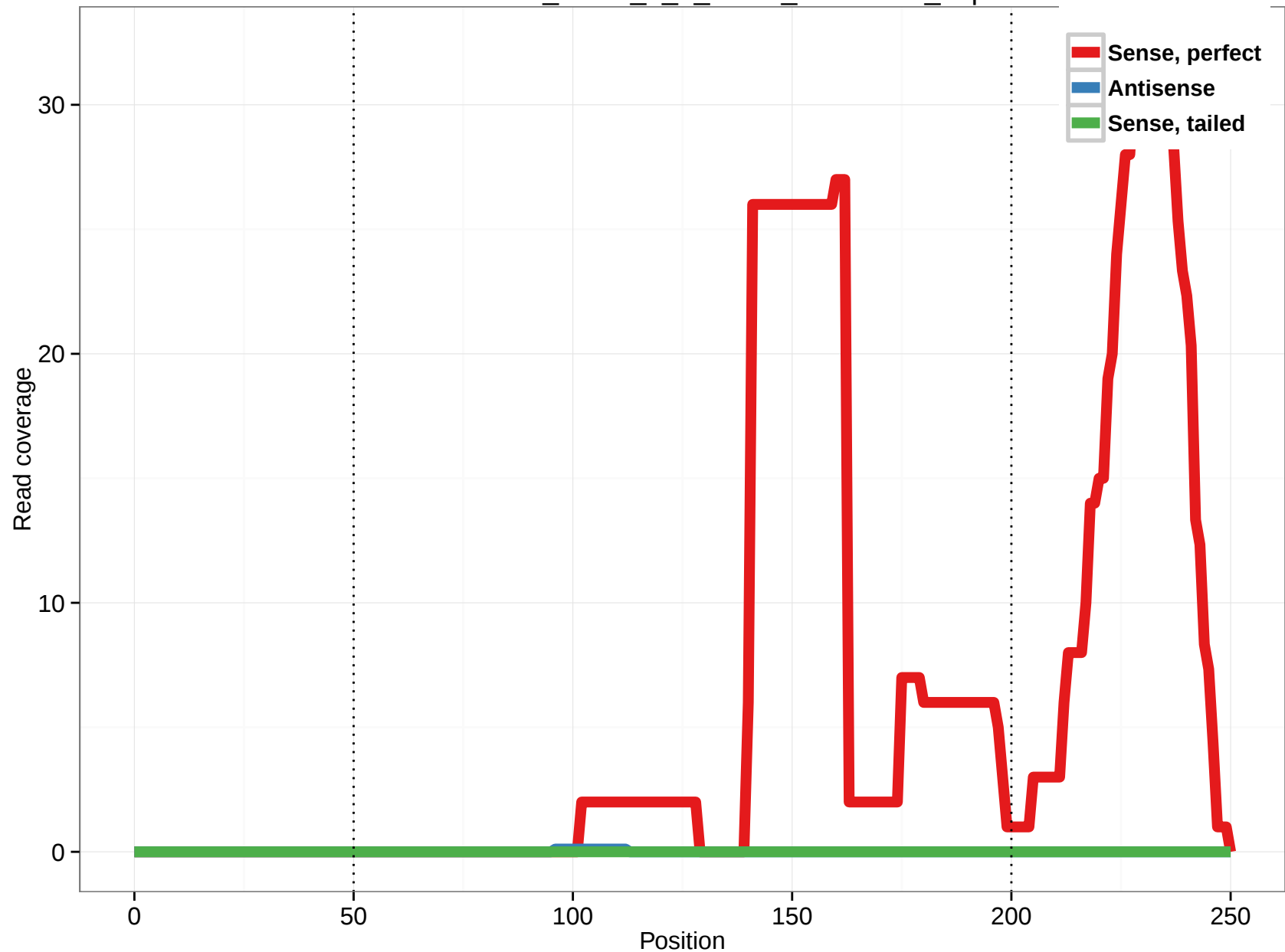
uc002mm.2_intron_3_0_chr19_10363378_f.3p
