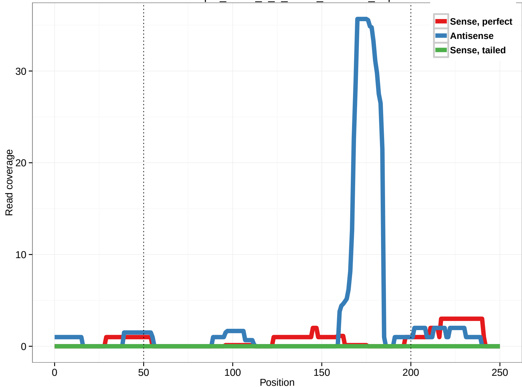
uc002mip.2_intron_1_0_chr19_7934795_r.3p
