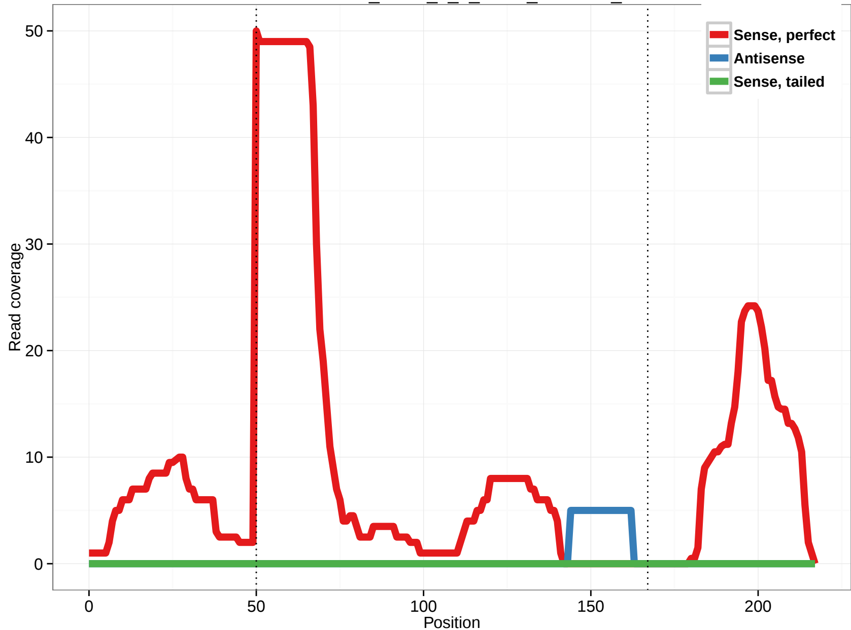
uc002mff.1_intron_1_0_chr19_6501409_r
