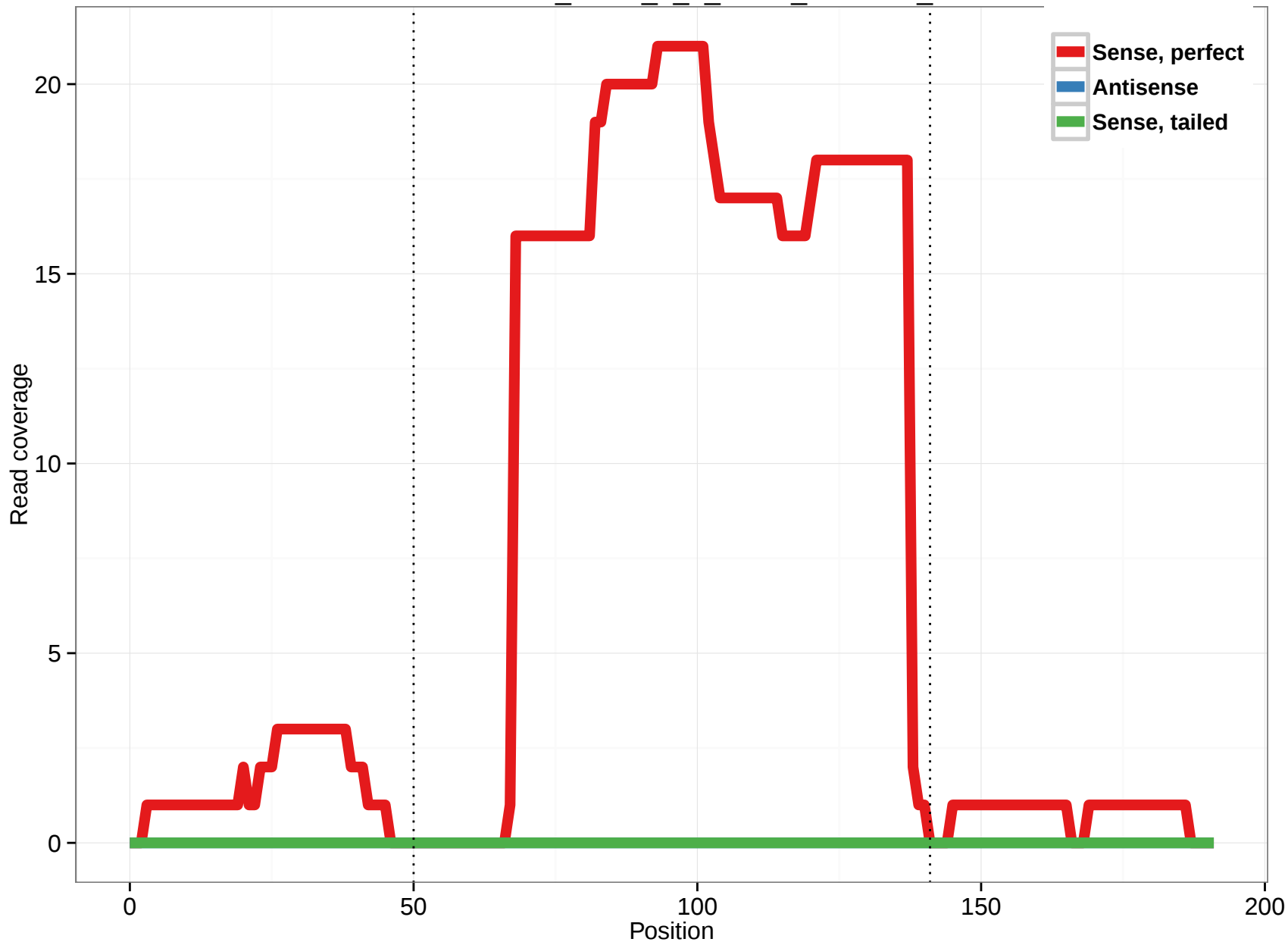
uc002mdc.2_intron_1_0_chr19_5785523_r
