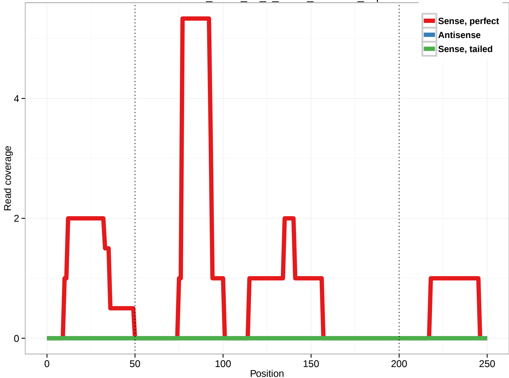
uc002lvb.3_intron_22_0_chr19_2220222_f.5p
