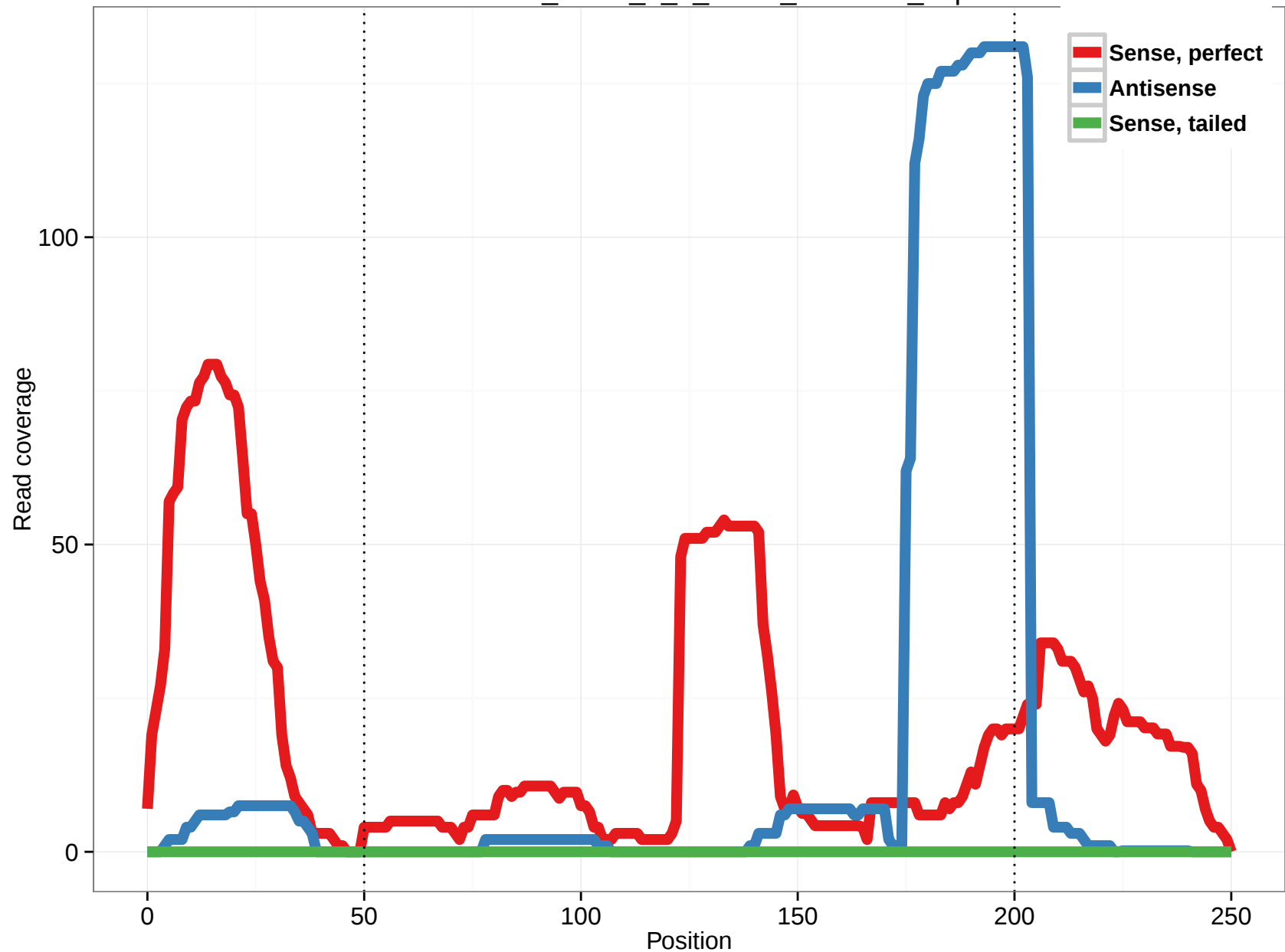
uc002lru.2_intron_5_0_chr19_1272051_f.5p
