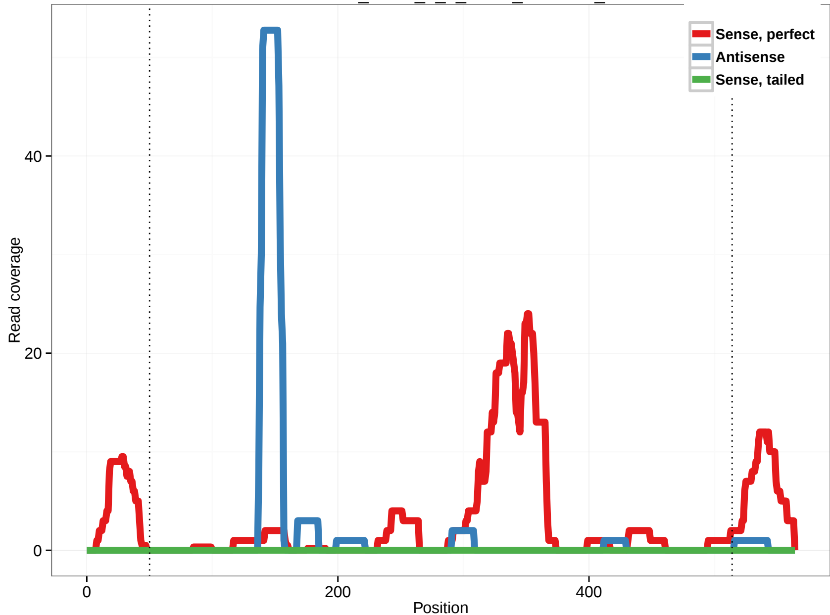
uc002ln.2_intron_0_0_chr19_1241991_f
