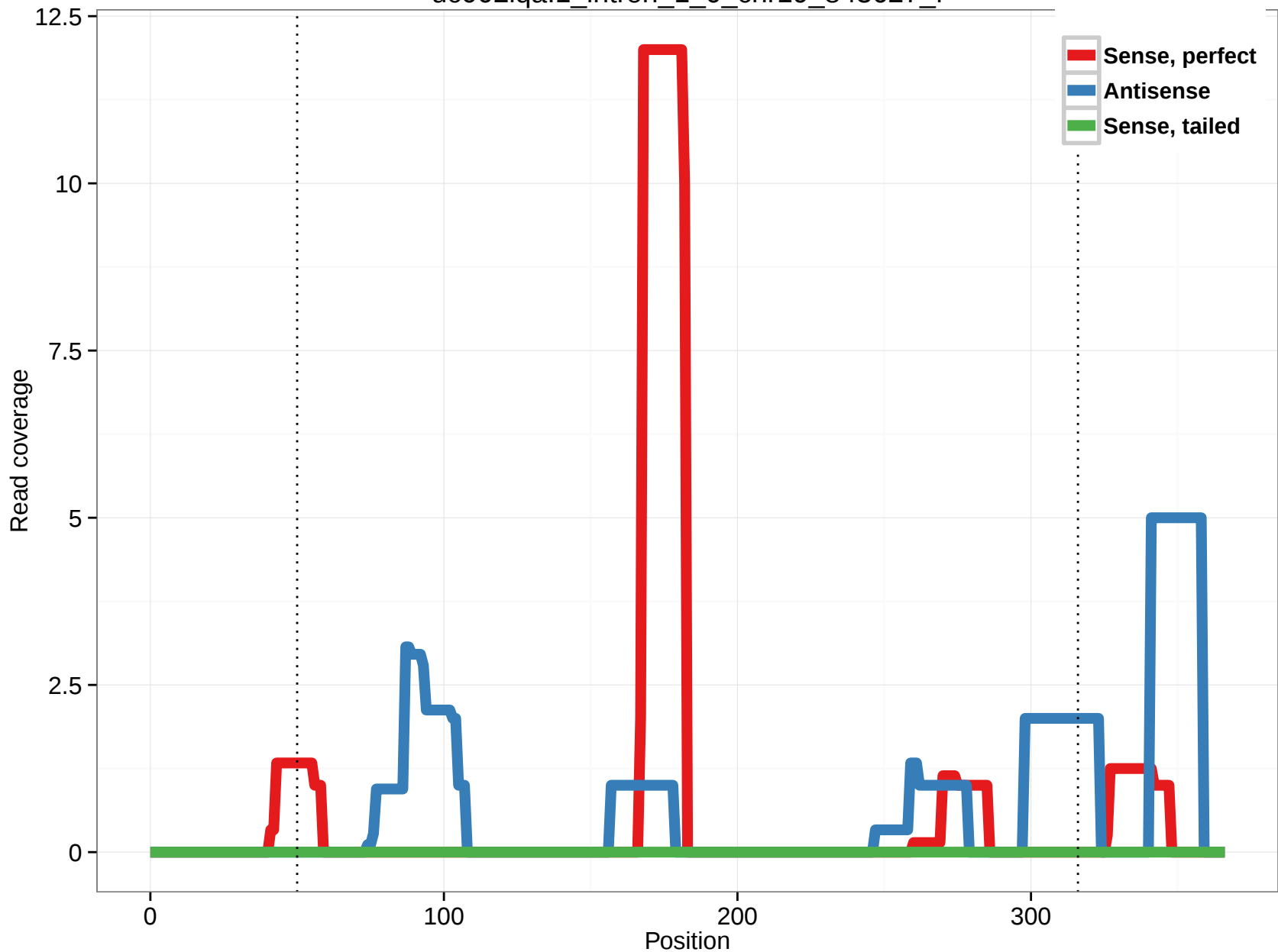
uc002lqa.1_intron_1_0_chr19_843627_f
