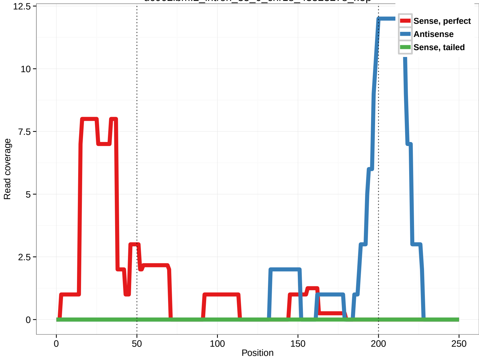
uc002lbm.2_intron_35_0_chr18_43523278_r.5p
