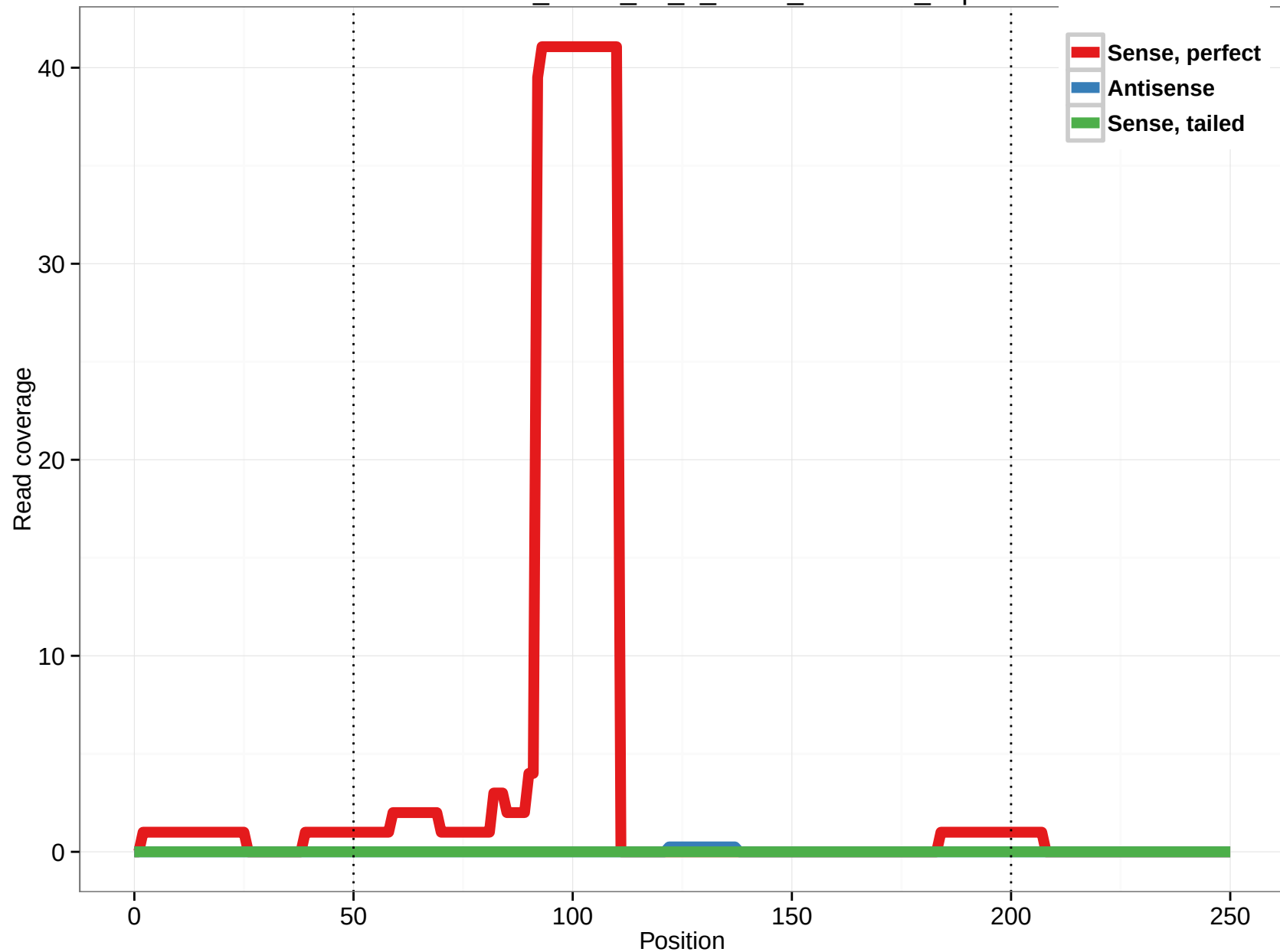
uc002klm.3_intron_34_0_chr18_2760738_f.5p
