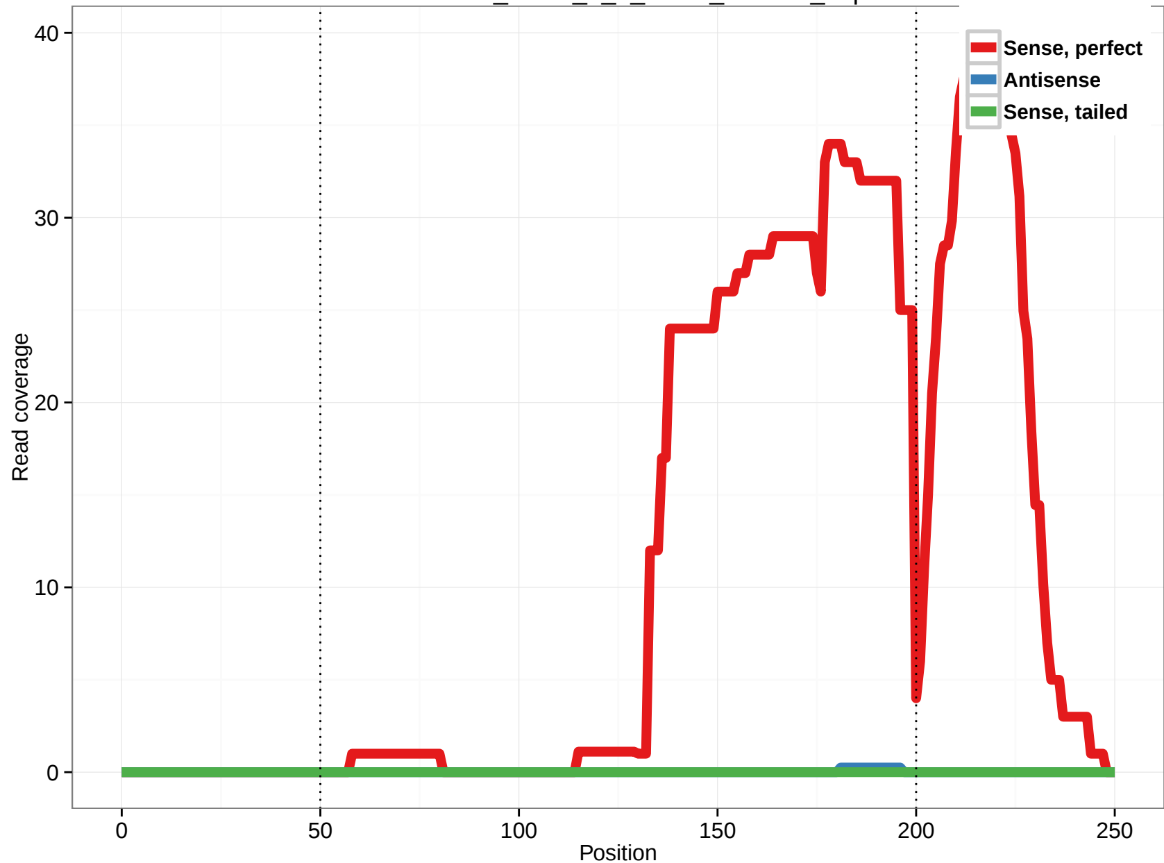
uc002kkf.1_intron_8_0_chr18_198133_f.3p
