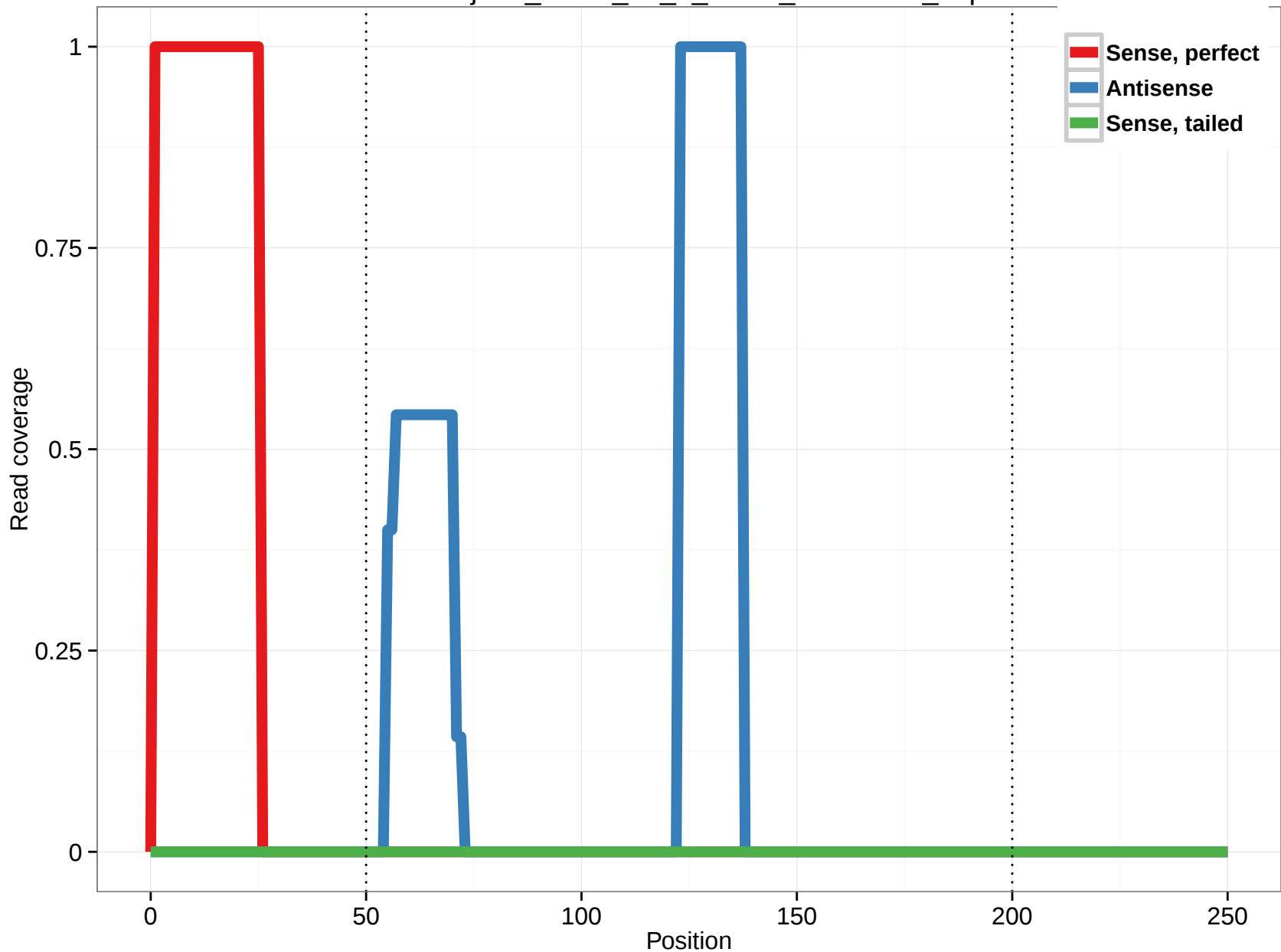
uc002jth.2_intron_14_0_chr17_74942533_f.5p
