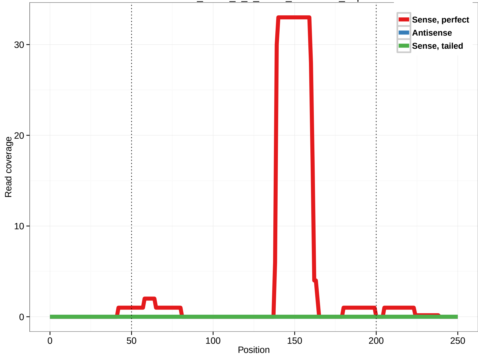
uc002ieh.2_intron_5_0_chr17_41891730_r.3p
