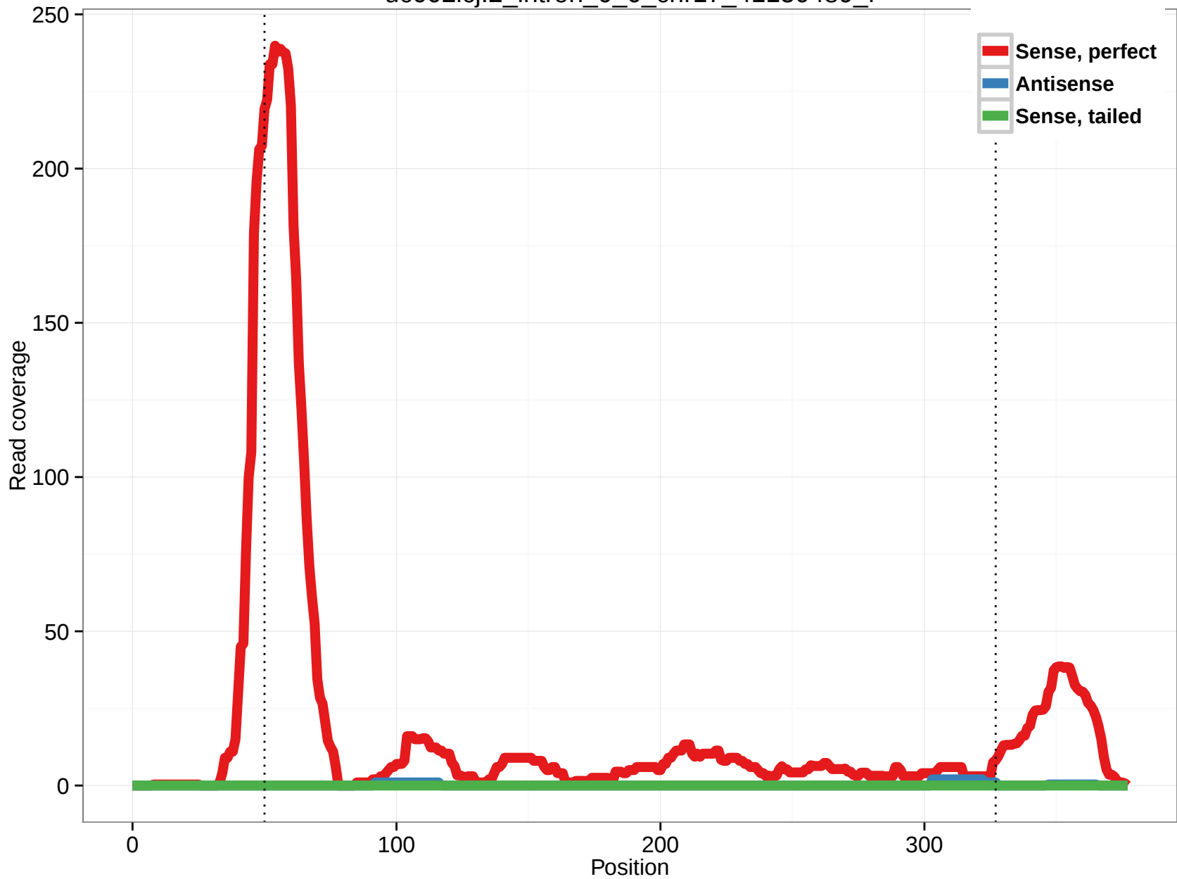
uc002icj.2_intron_0_0_chr17_41150489_f
