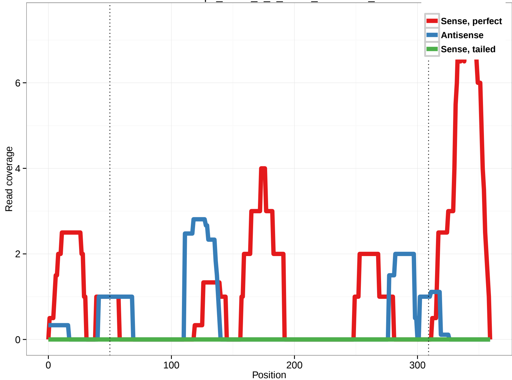
uc002iaq.2_intron_7_0_chr17_40817846_f
