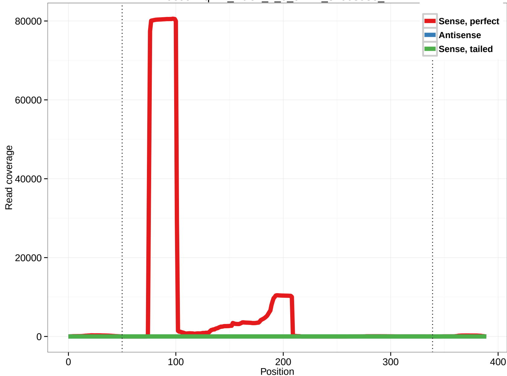
uc002hqw.1_intron_2_0_chr17_37008986_r
