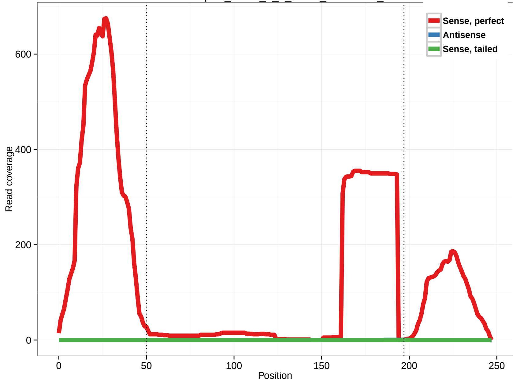
uc002hqw.1_intron_0_0_chr17_37006468_r
