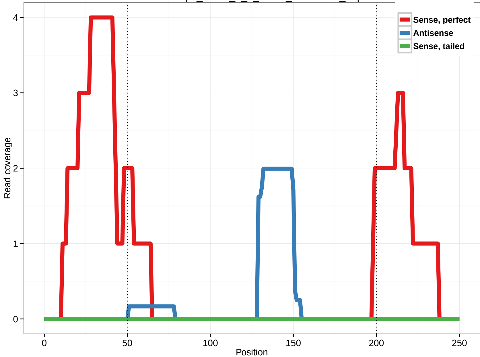
uc002hhq.2_intron_5_0_chr17_31263466_f.3p
