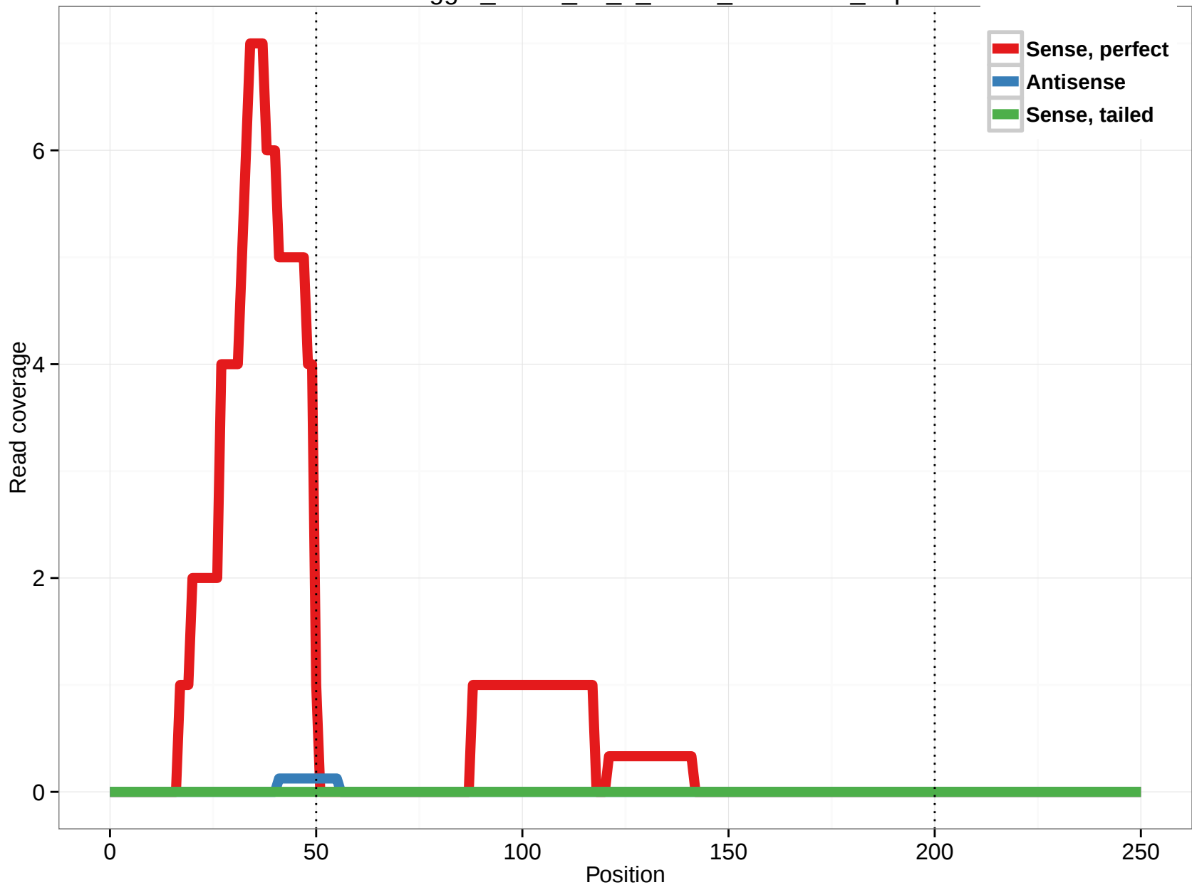
uc002hgg.2_intron_34_0_chr17_29588876_f.5p
