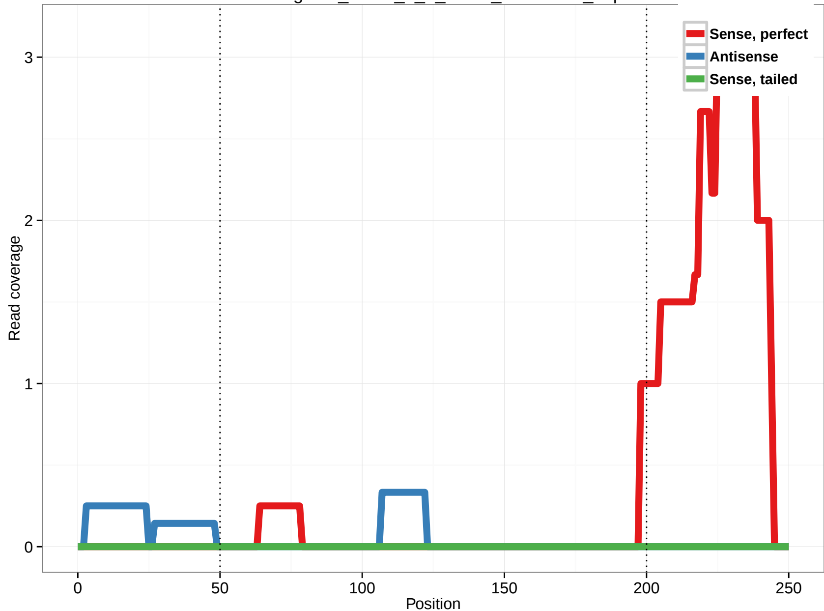
uc002gno.2_intron_5_0_chr17_12639654_f.3p
