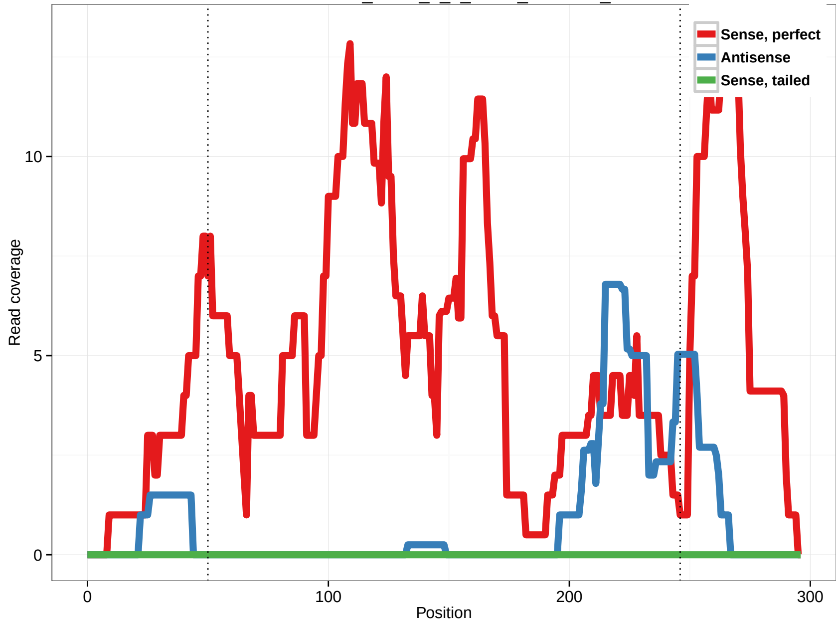
uc002fzv.2_intron_0_0_chr17_4844022_f
