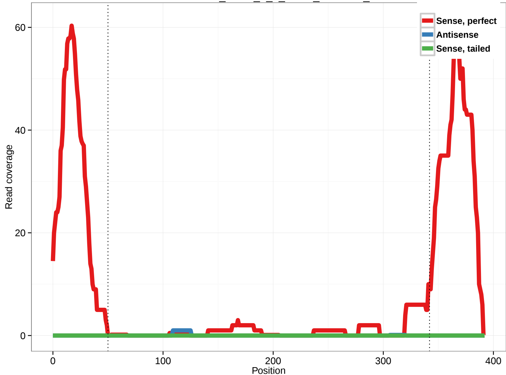
uc002fux.1_intron_9_0_chr17_2597859_r
