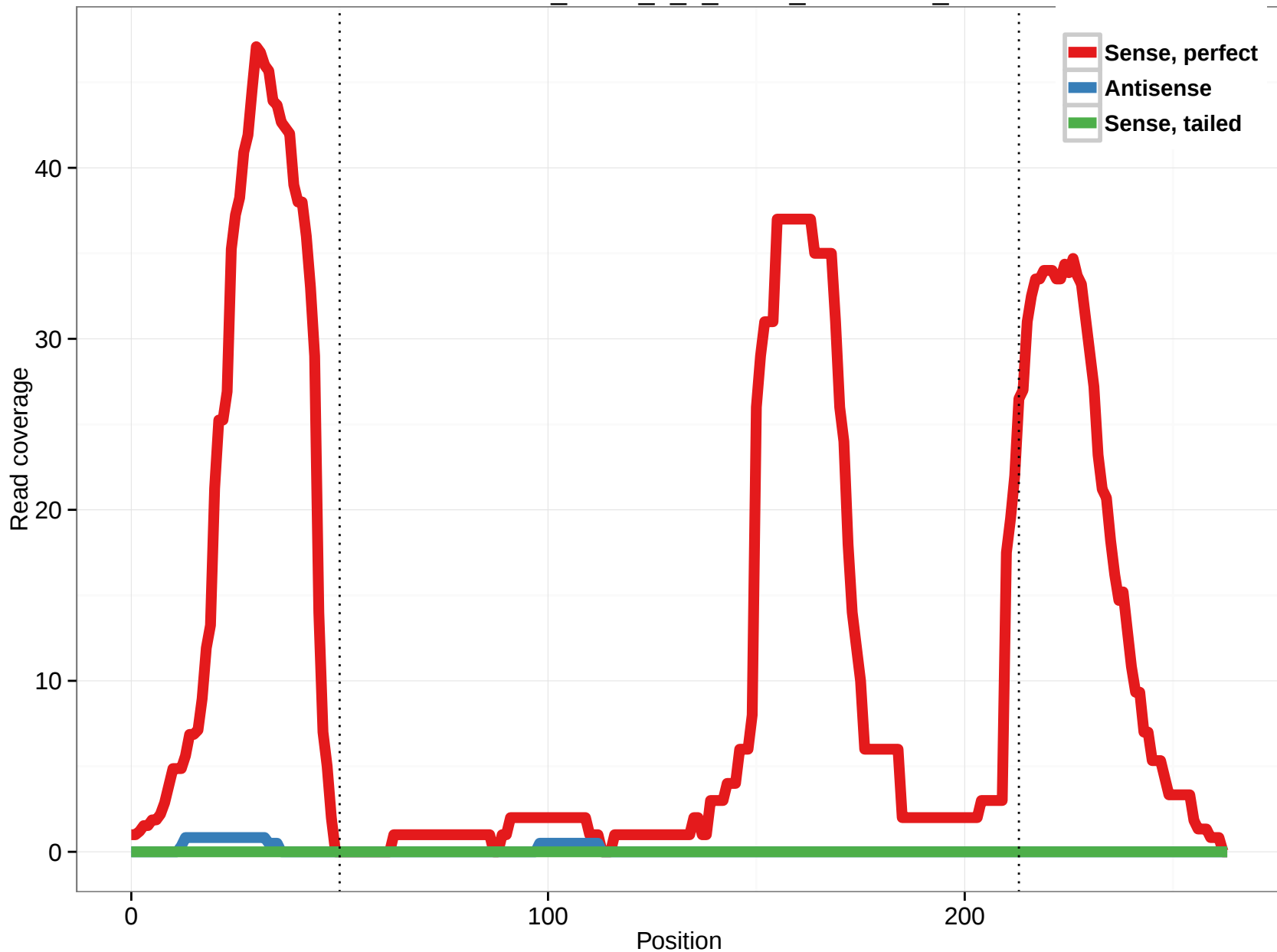
uc002fnm.1_intron_1_0_chr16_89627472_f
