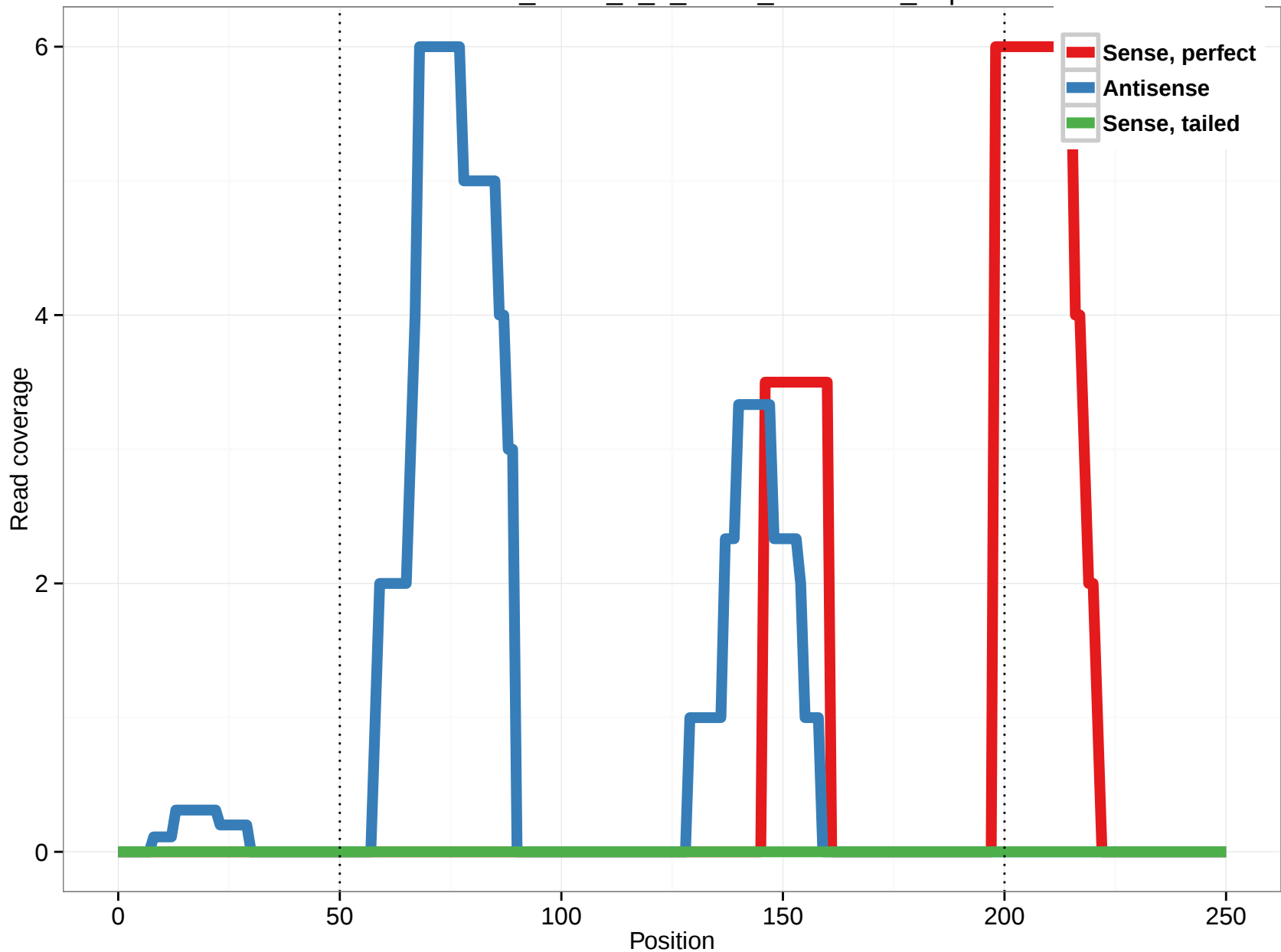
uc002fml.1_intron_5_0_chr16_88951678_r.3p
