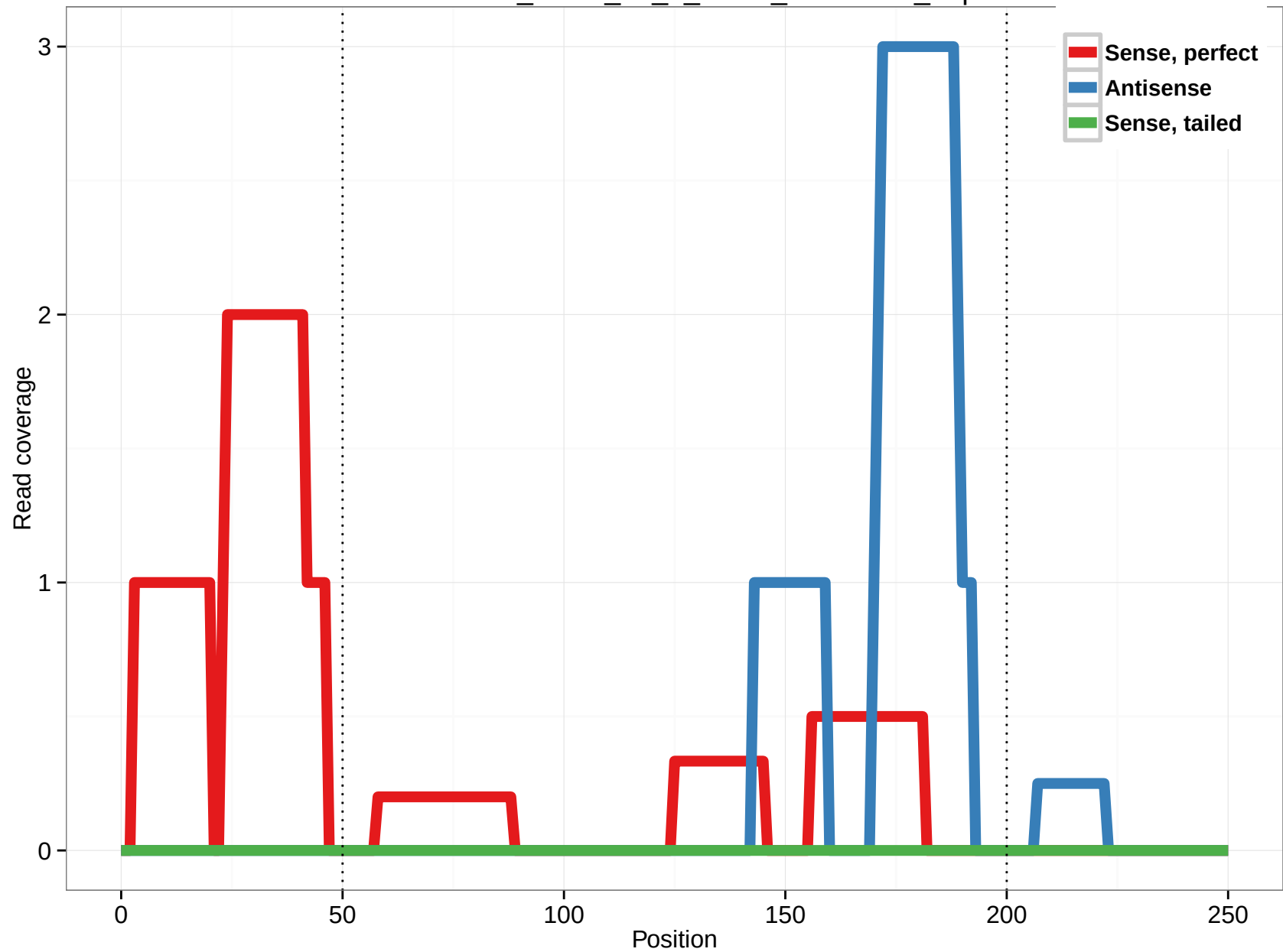
uc002ezc.2_intron_15_0_chr16_70548413_r.5p
