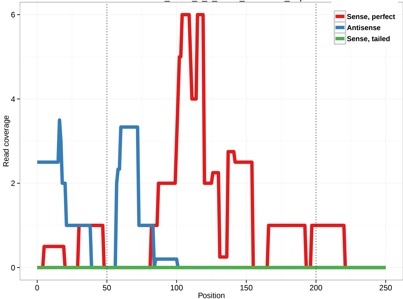
uc002eza.2_intron_4_0_chr16_70516725_r.5p
