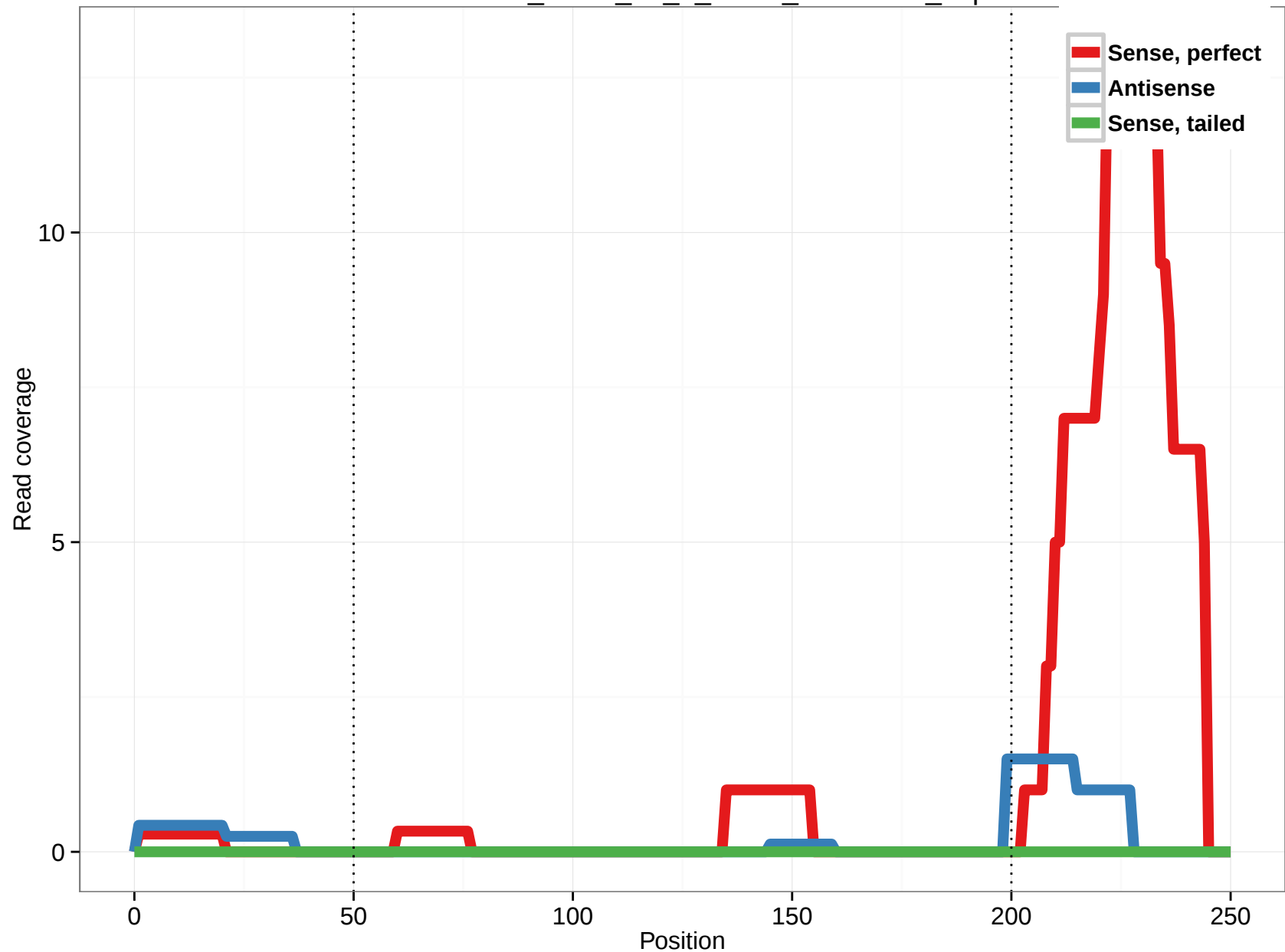
uc002ews.3_intron_15_0_chr16_69201089_f.3p
