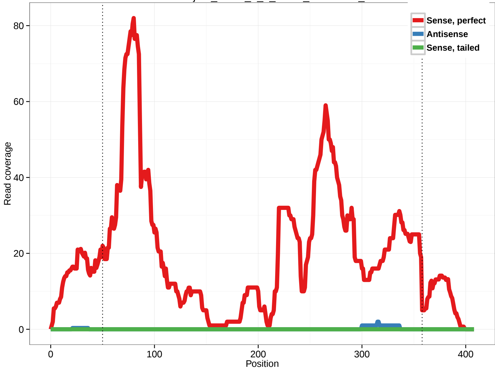
uc002ejh.2_intron_0_0_chr16_56642596_f
