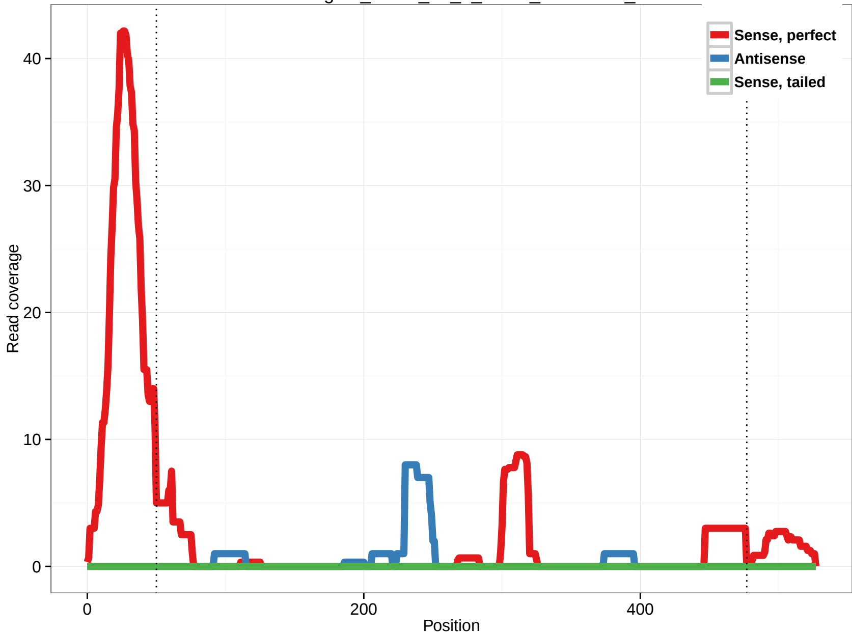
uc002ege.1_intron_15_0_chr16_50402210_r
