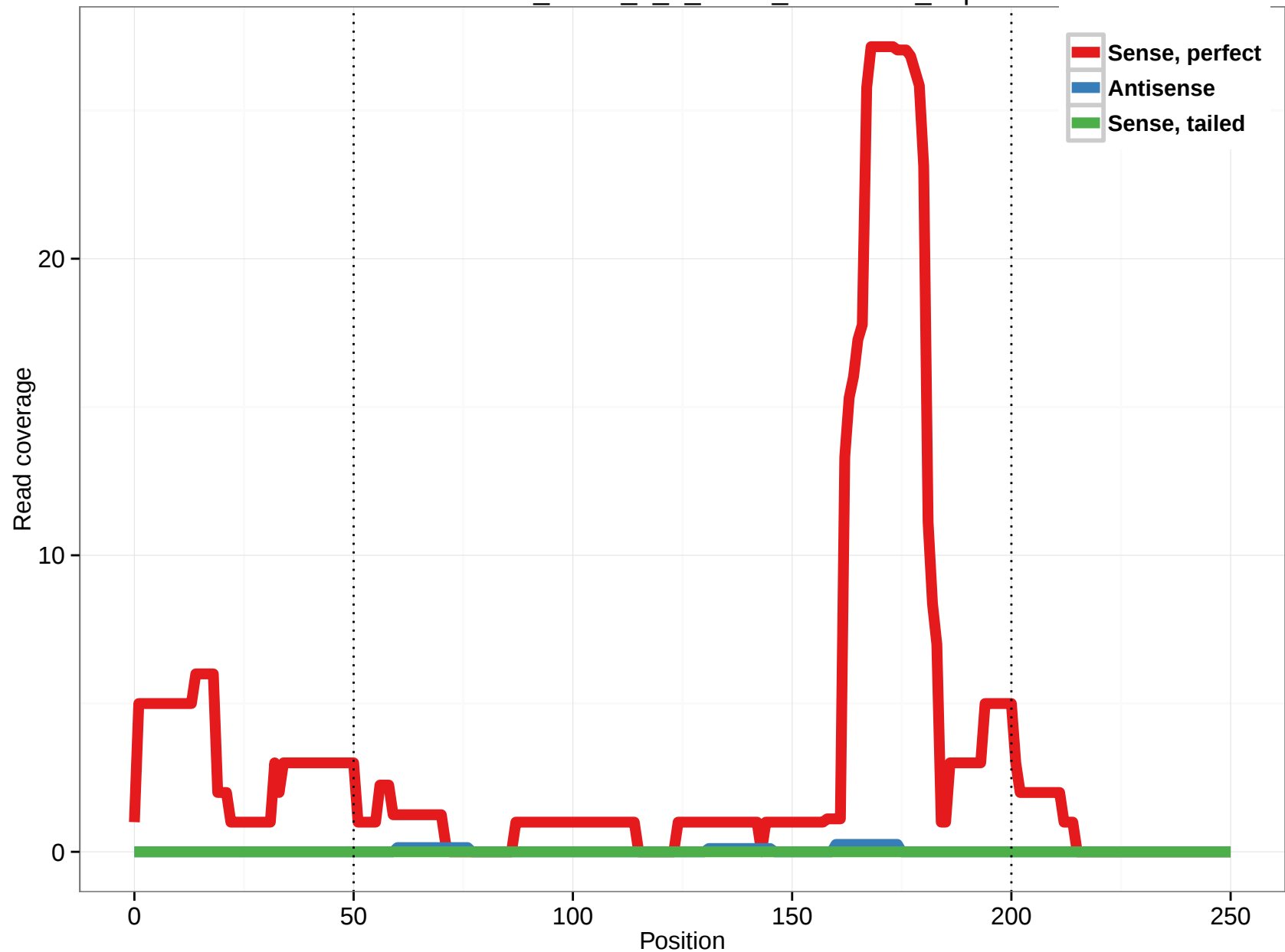
uc002eek.1_intron_2_0_chr16_46858395_r.5p
