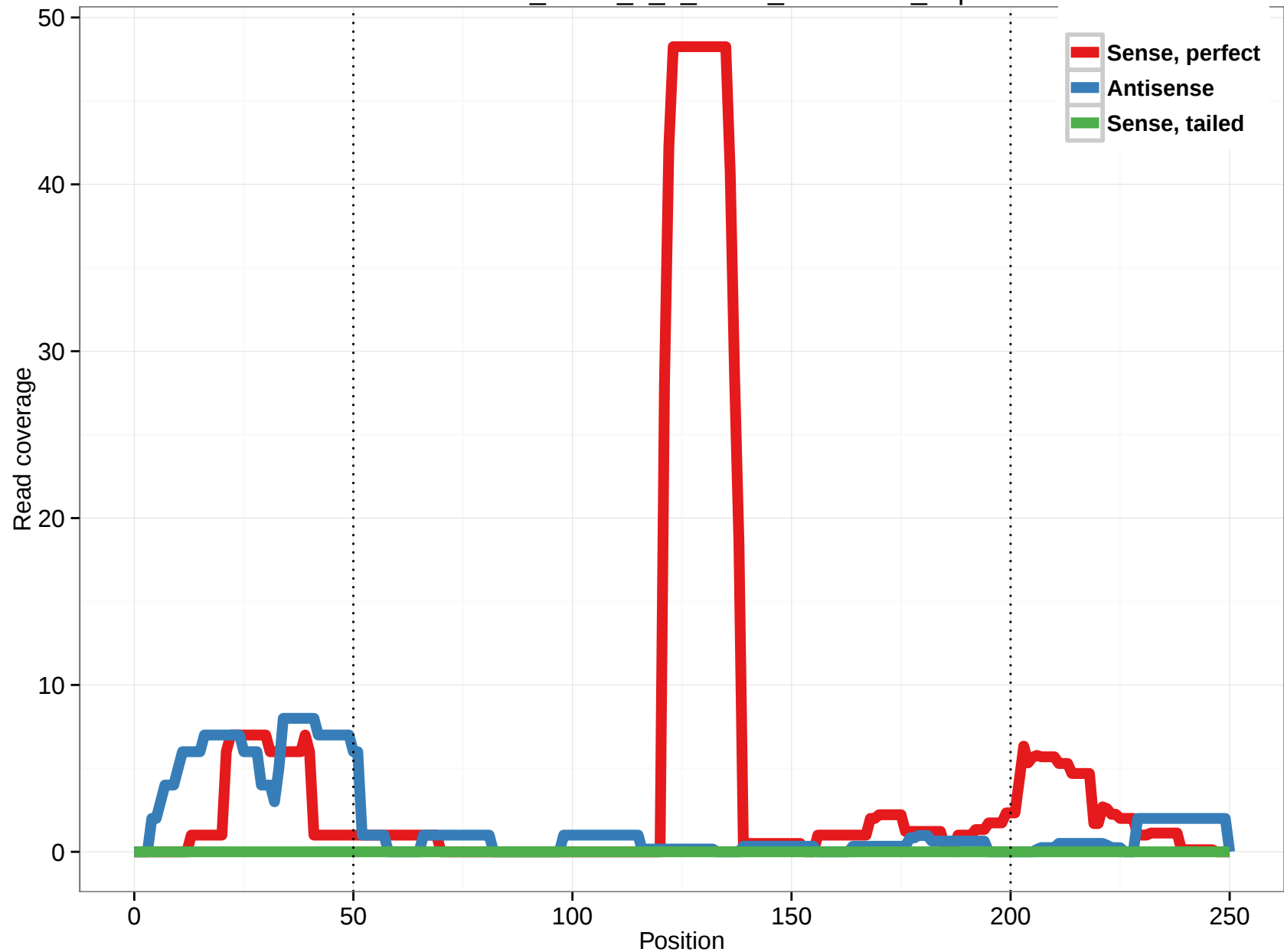
uc002dtv.1_intron_0_0_chr16_29817502_f.5p
