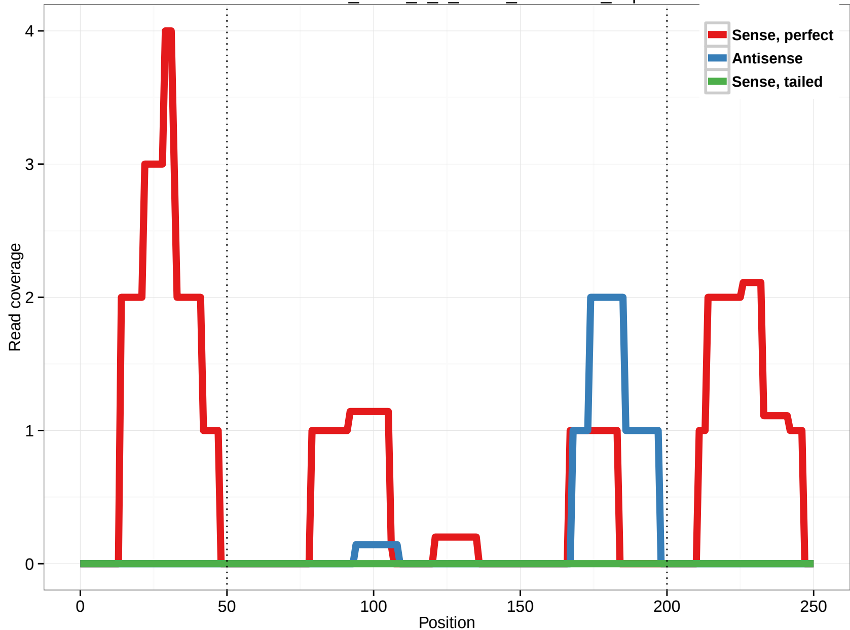
uc002dox.1_intron_8_0_chr16_27715320_f.5p
