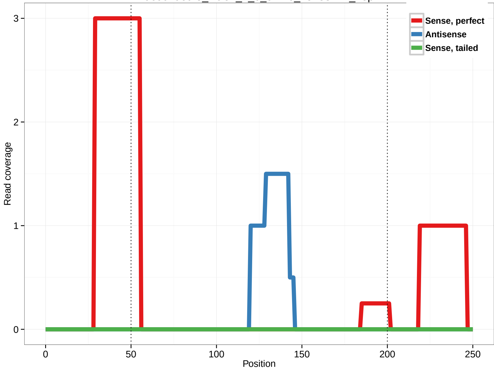
uc002dod.3_intron_2_0_chr16_25258712_r.3p
